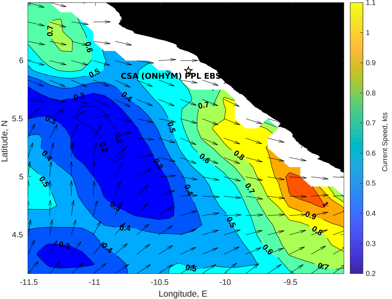
Surface Currents for CSA (ONHYM) PPL EBS - Liberia at 18-Oct-2025 00:00:00
