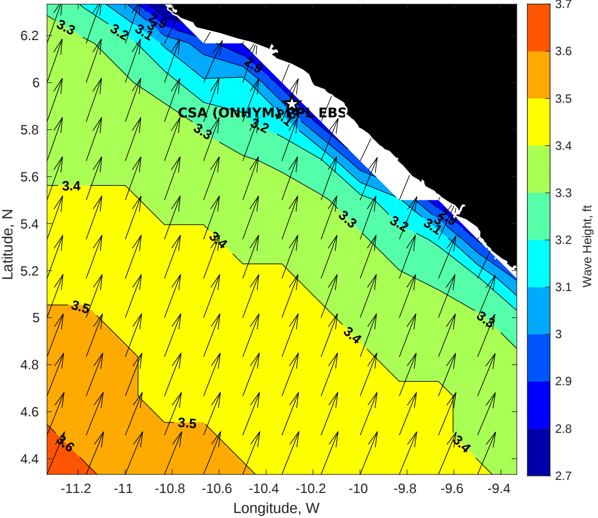
Wave Height (ft) for CSA (ONHYM) PPL EBS - Liberia at 19-Oct-2025 09:00:00
