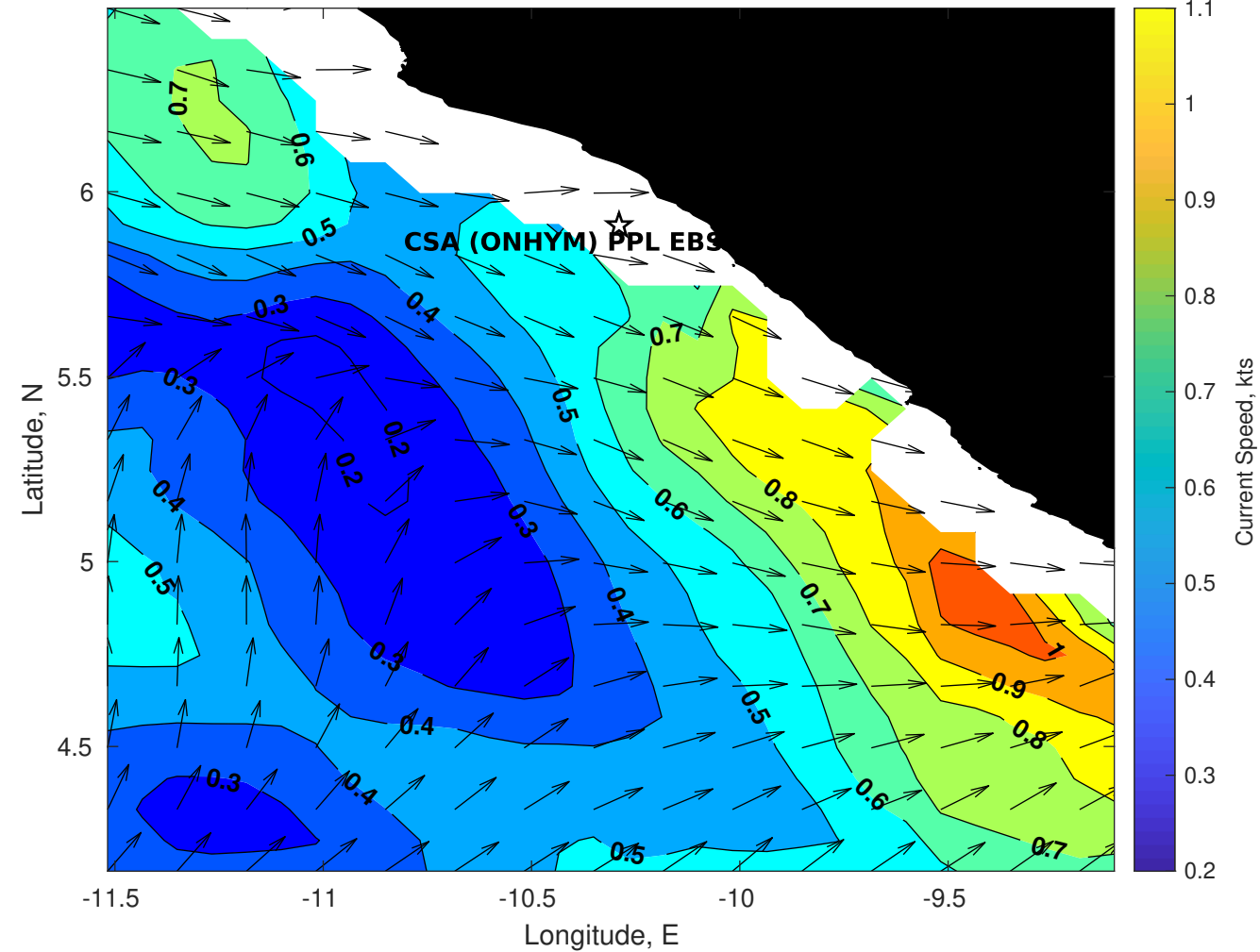
Surface Currents for CSA (ONHYM) PPL EBS - Liberia at 18-Oct-2025 00:00:00
