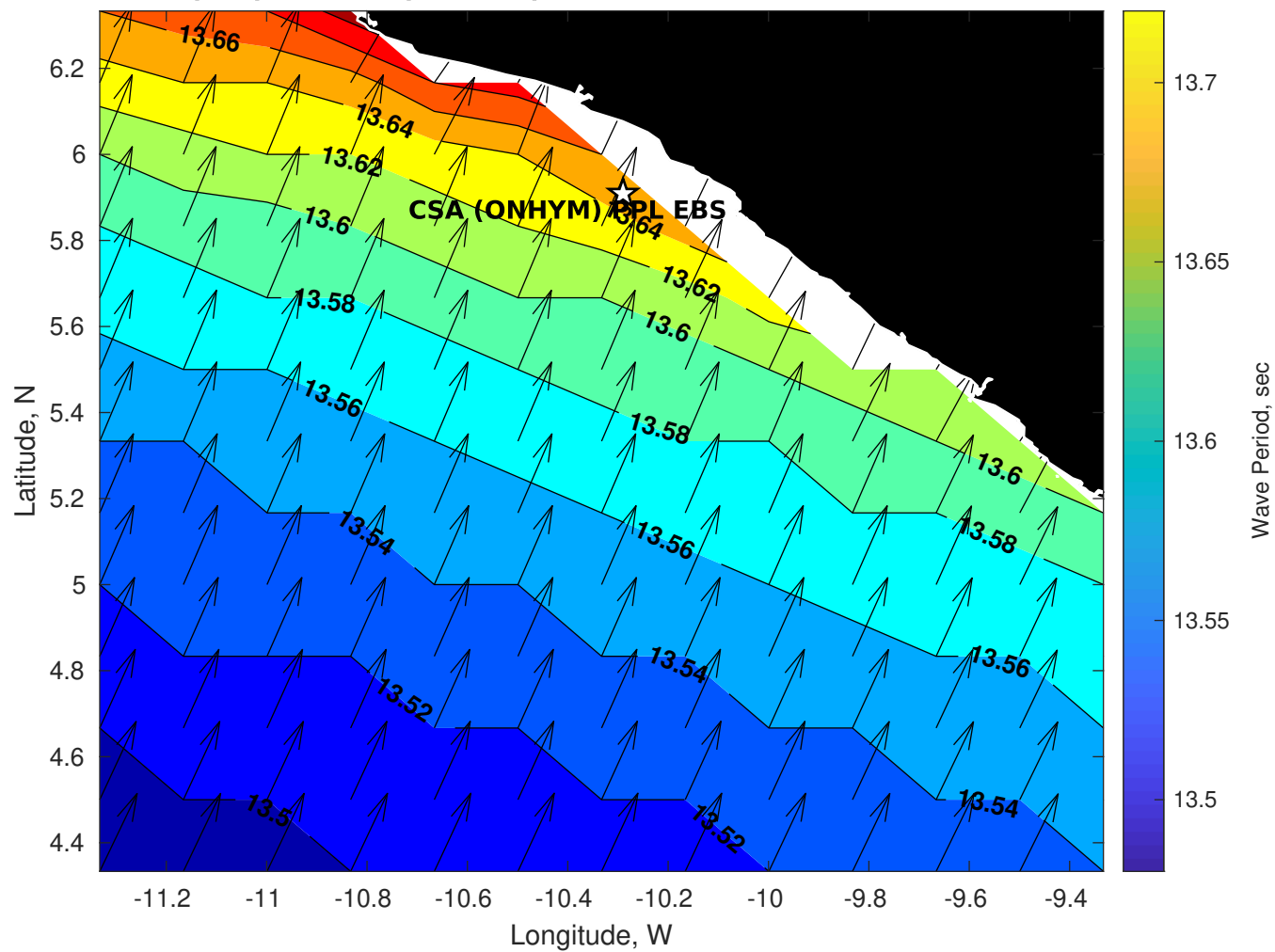
Wave Period (sec) for CSA (ONHYM) PPL EBS - Liberia at 19-Oct-2025 09:00:00
