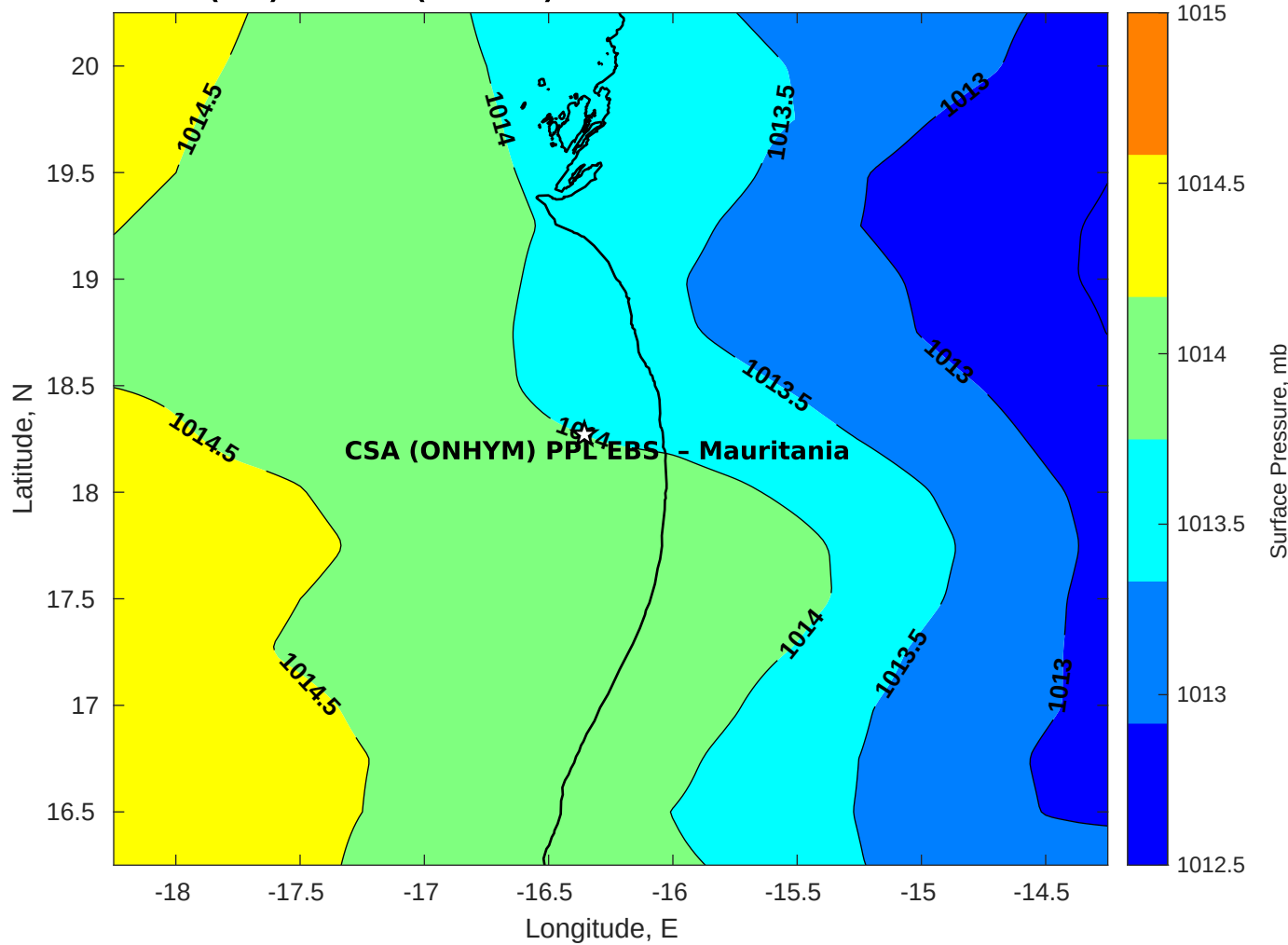
Surface Pressure (mb) for CSA (ONHYM) PPL EBS - Mauritania at 19-Oct-2025 00:00:00
