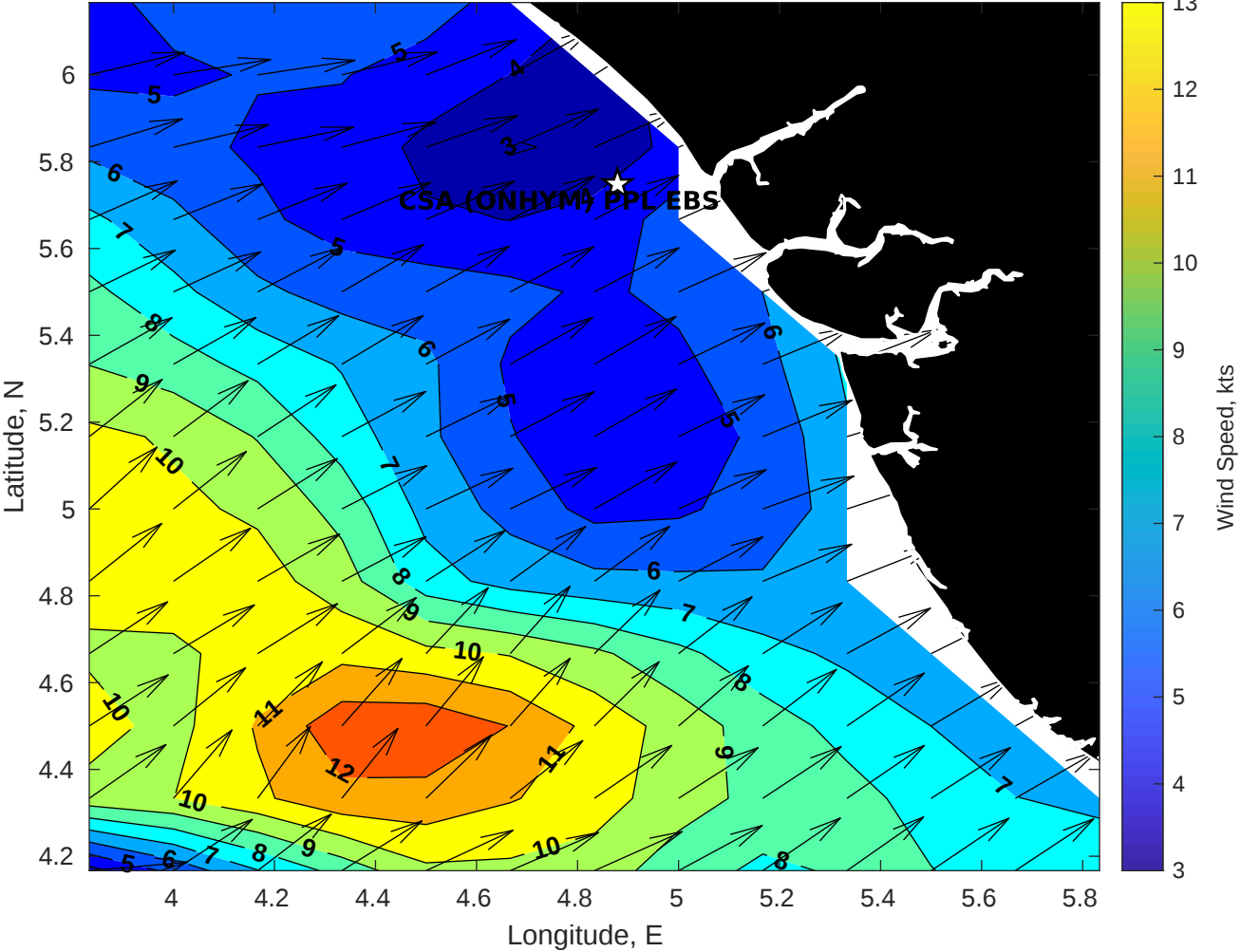
Winds (kts) for CSA (ONHYM) PPL EBS - Nigeria at 19-Oct-2025 09:00:00
