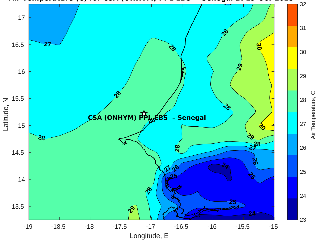
Air Temperature (C) for CSA (ONHYM) PPL EBS - Senegal at 19-Oct-2025
