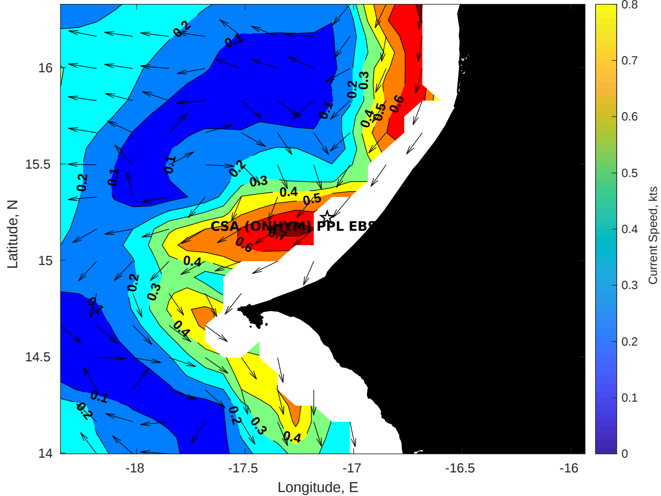
Surface Currents for CSA (ONHYM) PPL EBS - Senegal at 18-Oct-2025 00:00:00
