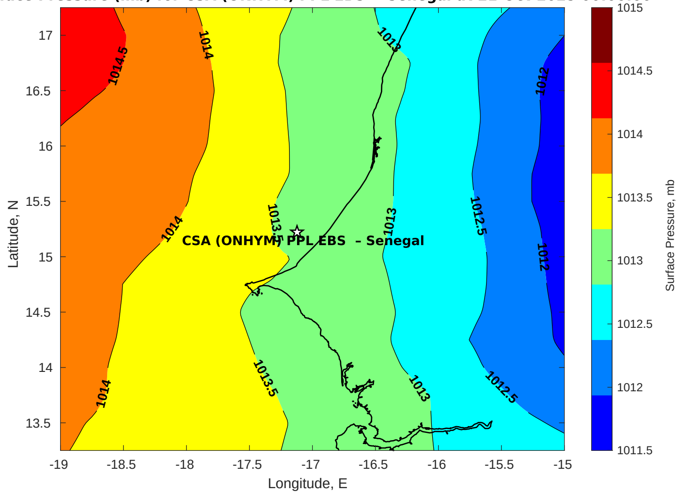
Surface Pressure (mb) for CSA (ONHYM) PPL EBS - Senegal at 21-Oct-2025 00:00:00
