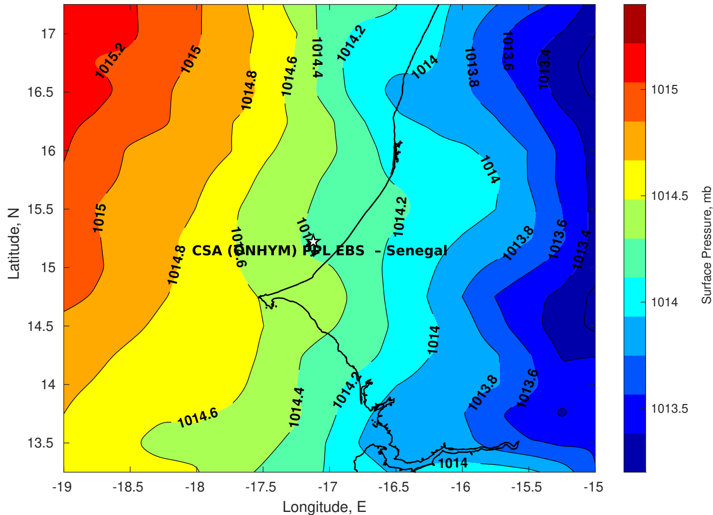
Surface Pressure (mb) for CSA (ONHYM) PPL EBS - Senegal at 20-Oct-2025 00:00:00
