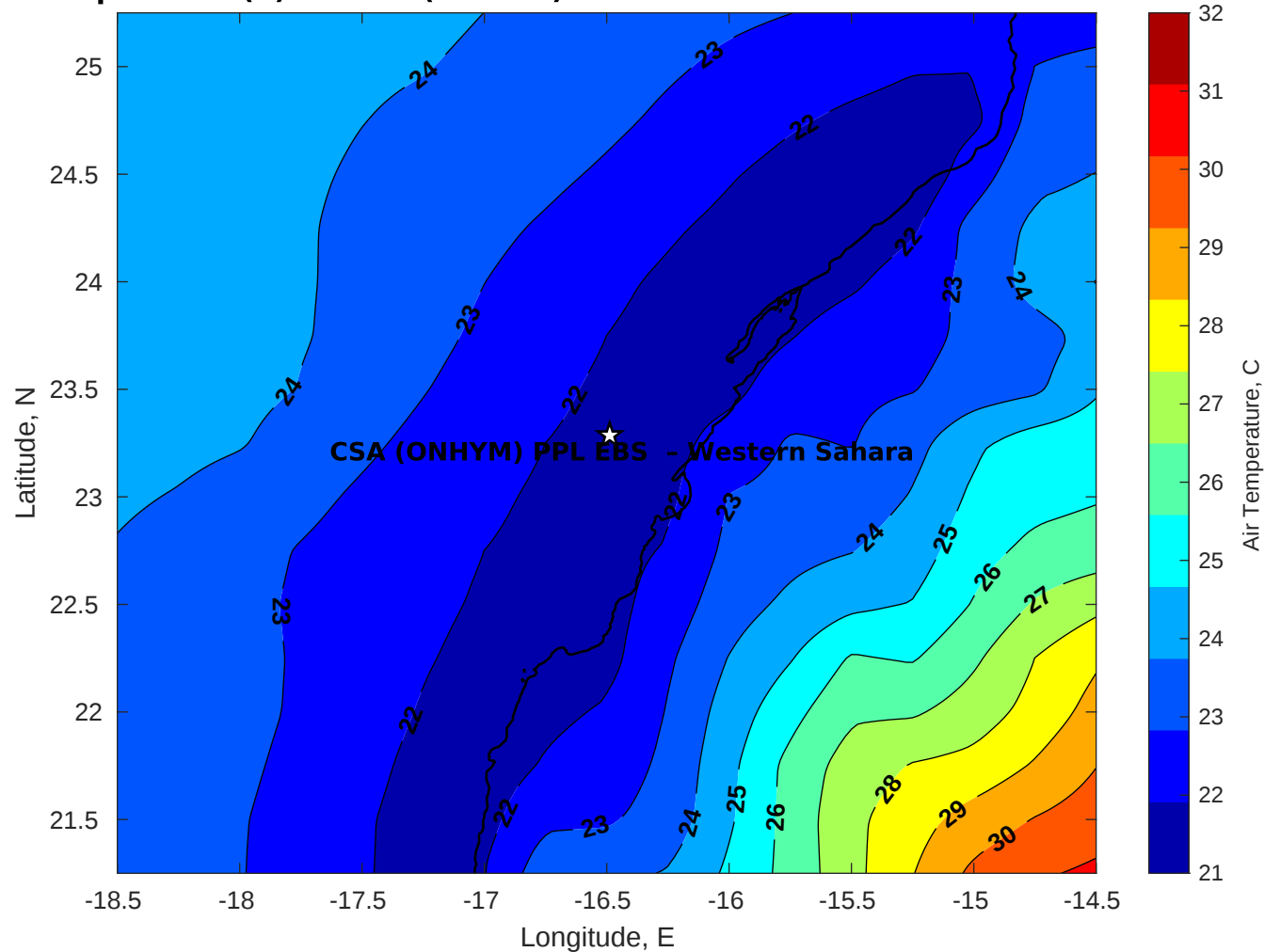
Air Temperature (C) for CSA (ONHYM) PPL EBS - Western Sahara at 19-Oct-2025
