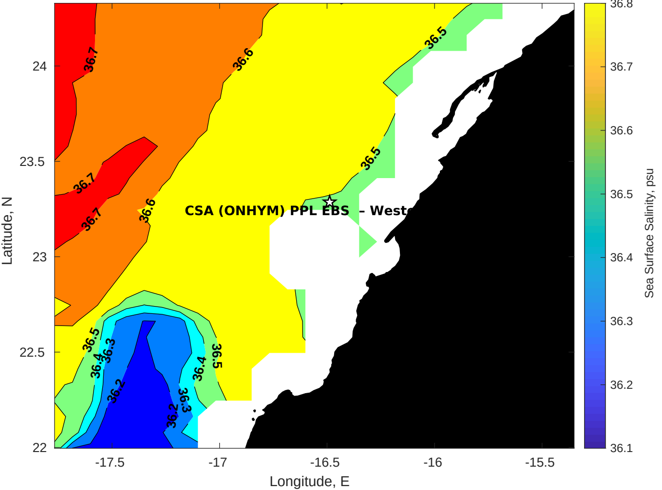
Surface Salinity for CSA (ONHYM) PPL EBS - Western Sahara at 16-Oct-2025 00:00:00
