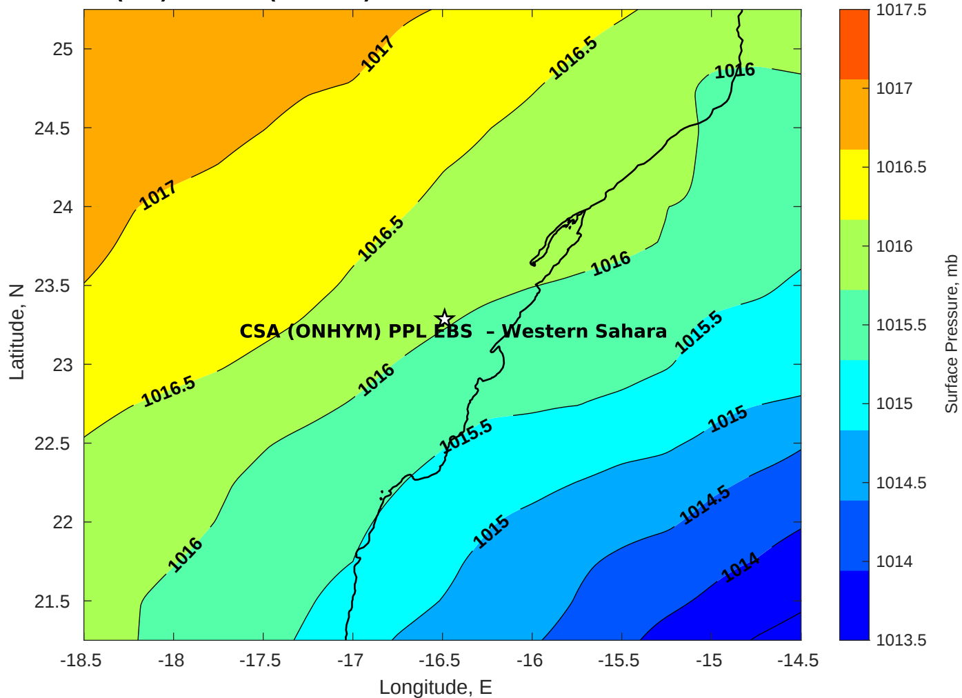
Surface Pressure (mb) for CSA (ONHYM) PPL EBS - Western Sahara at 20-Oct-2025 00:00:00
