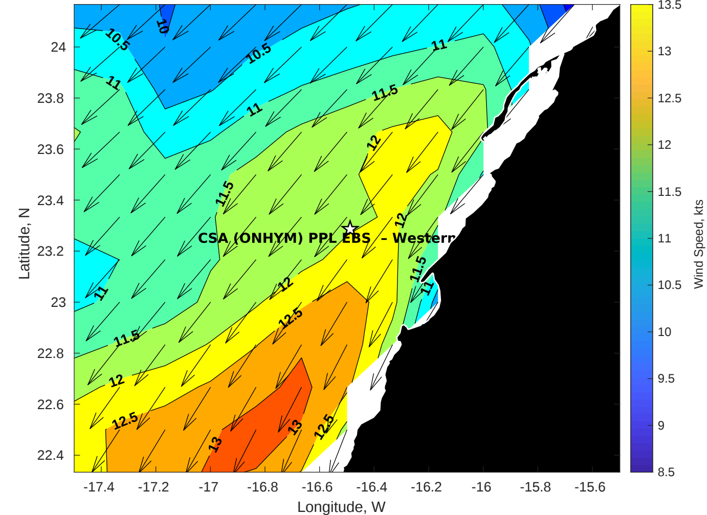
Winds (kts) for CSA (ONHYM) PPL EBS - Western Sahara at 19-Oct-2025 09:00:00
