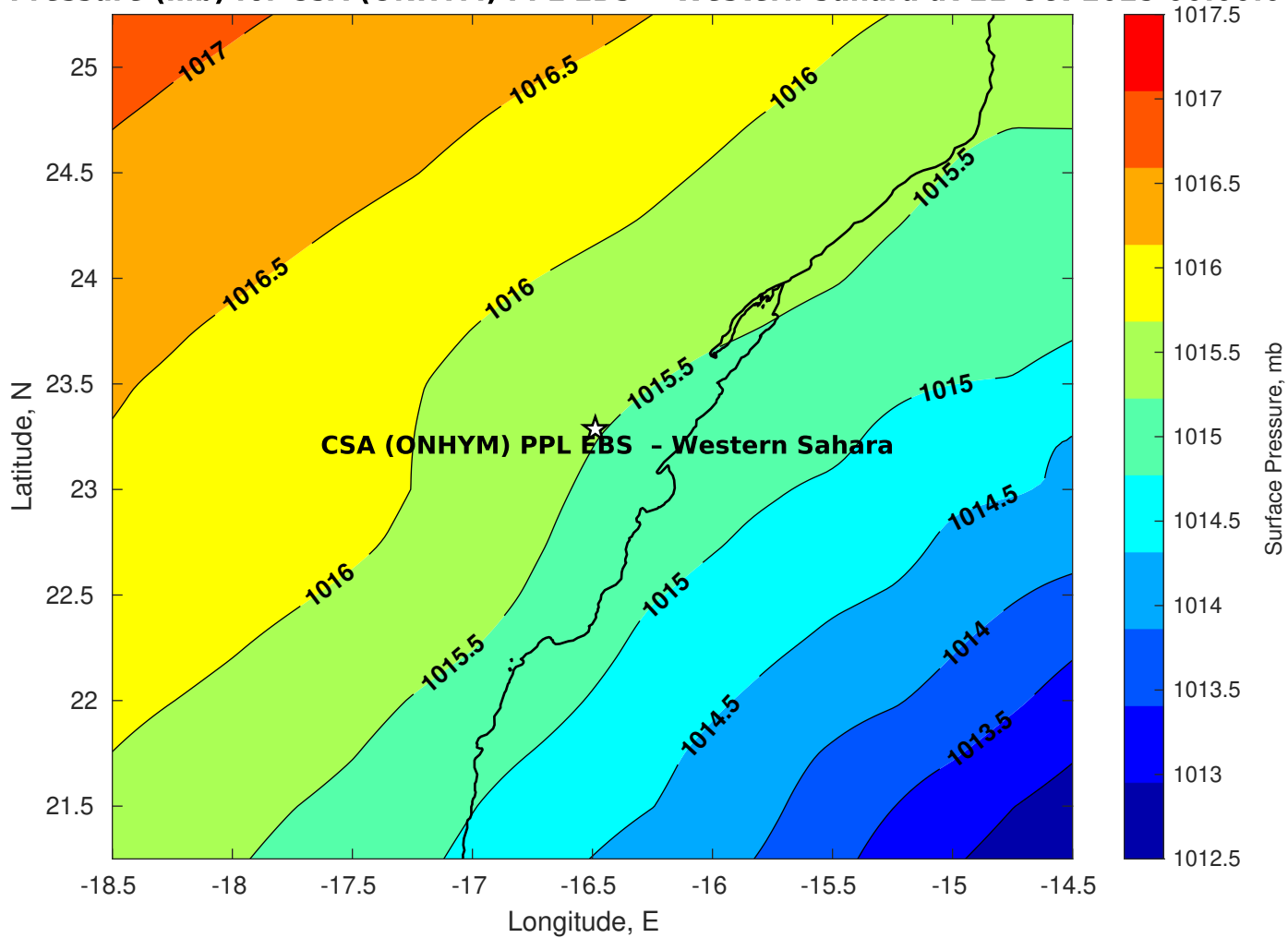
Surface Pressure (mb) for CSA (ONHYM) PPL EBS - Western Sahara at 21-Oct-2025 00:00:00
