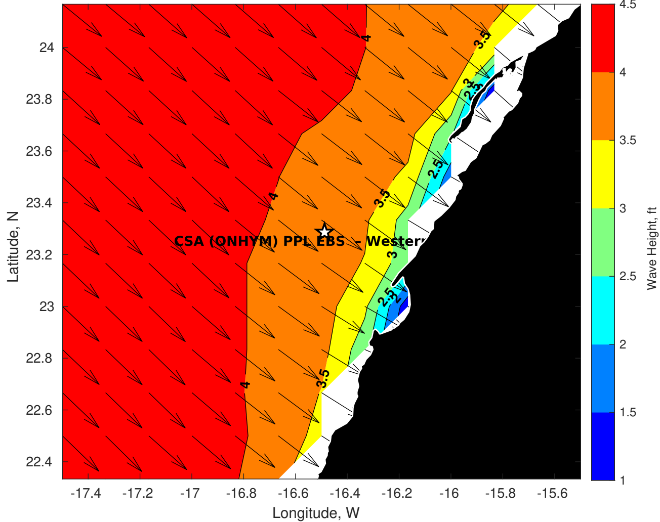
Wave Height (ft) for CSA (ONHYM) PPL EBS - Western Sahara at 19-Oct-2025 09:00:00
