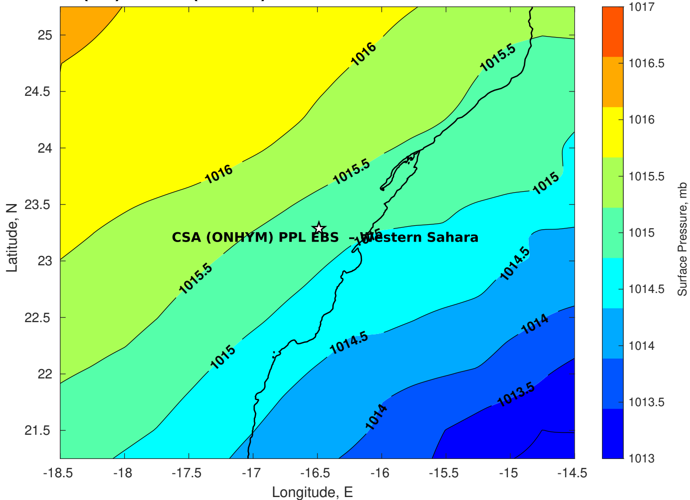
Surface Pressure (mb) for CSA (ONHYM) PPL EBS - Western Sahara at 19-Oct-2025 00:00:00
