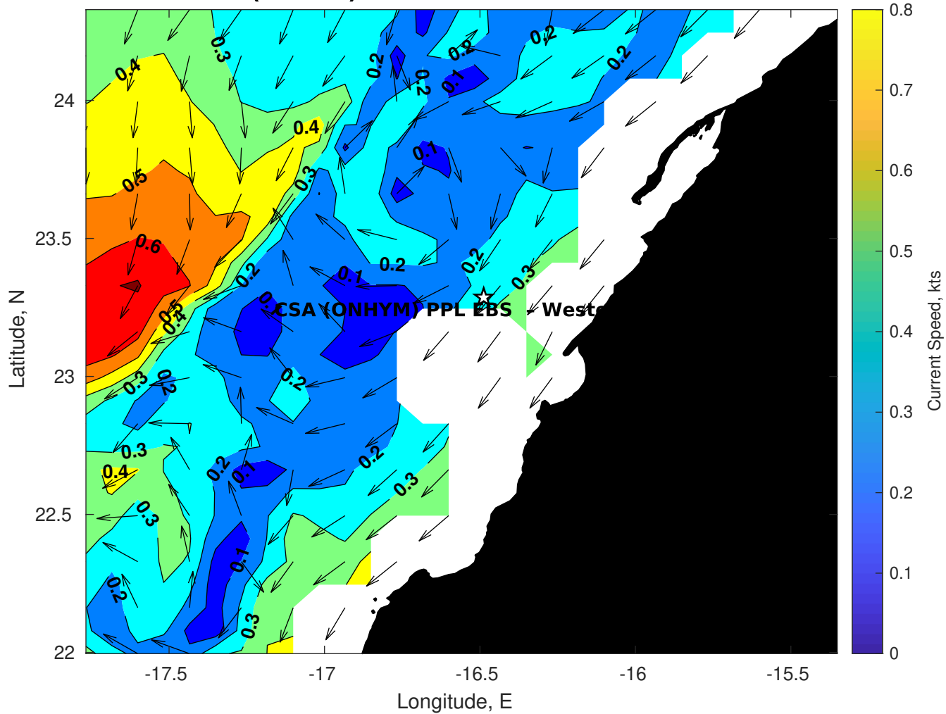
Surface Currents for CSA (ONHYM) PPL EBS - Western Sahara at 16-Oct-2025 00:00:00
