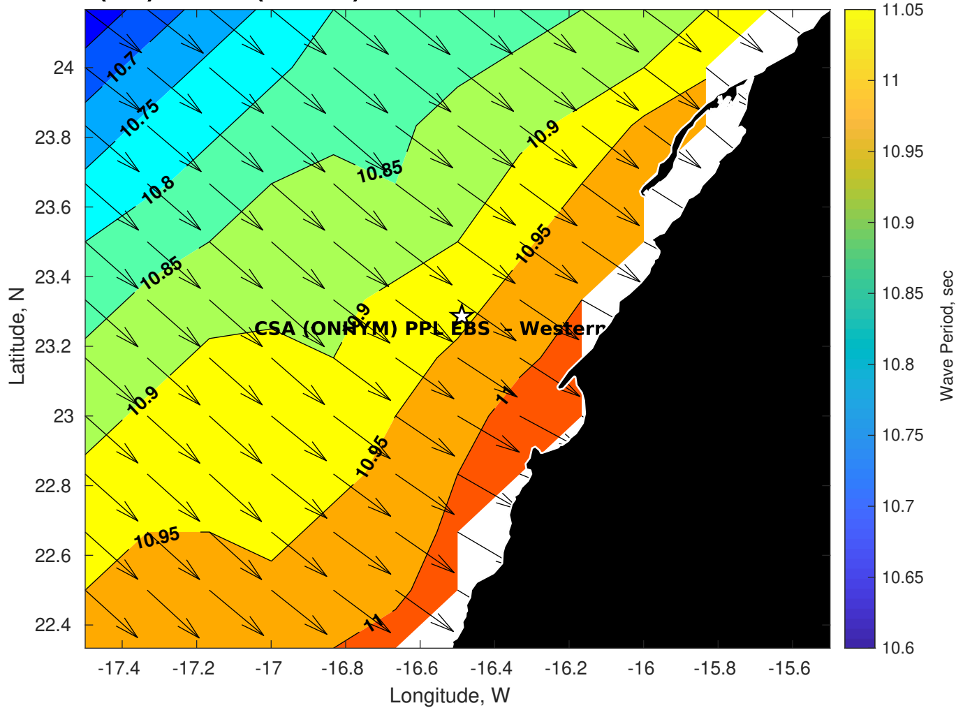
Wave Period (sec) for CSA (ONHYM) PPL EBS - Western Sahara at 19-Oct-2025 09:00:00
