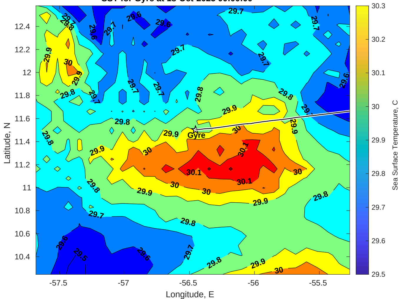
SST for Gyre at 18-Oct-2025 00:00:00
