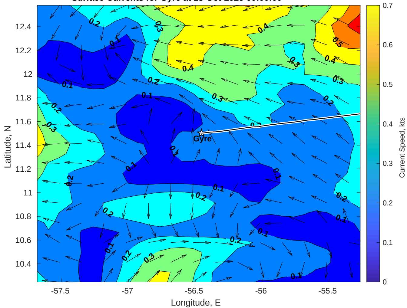
Surface Currents for Gyre at 18-Oct-2025 00:00:00
