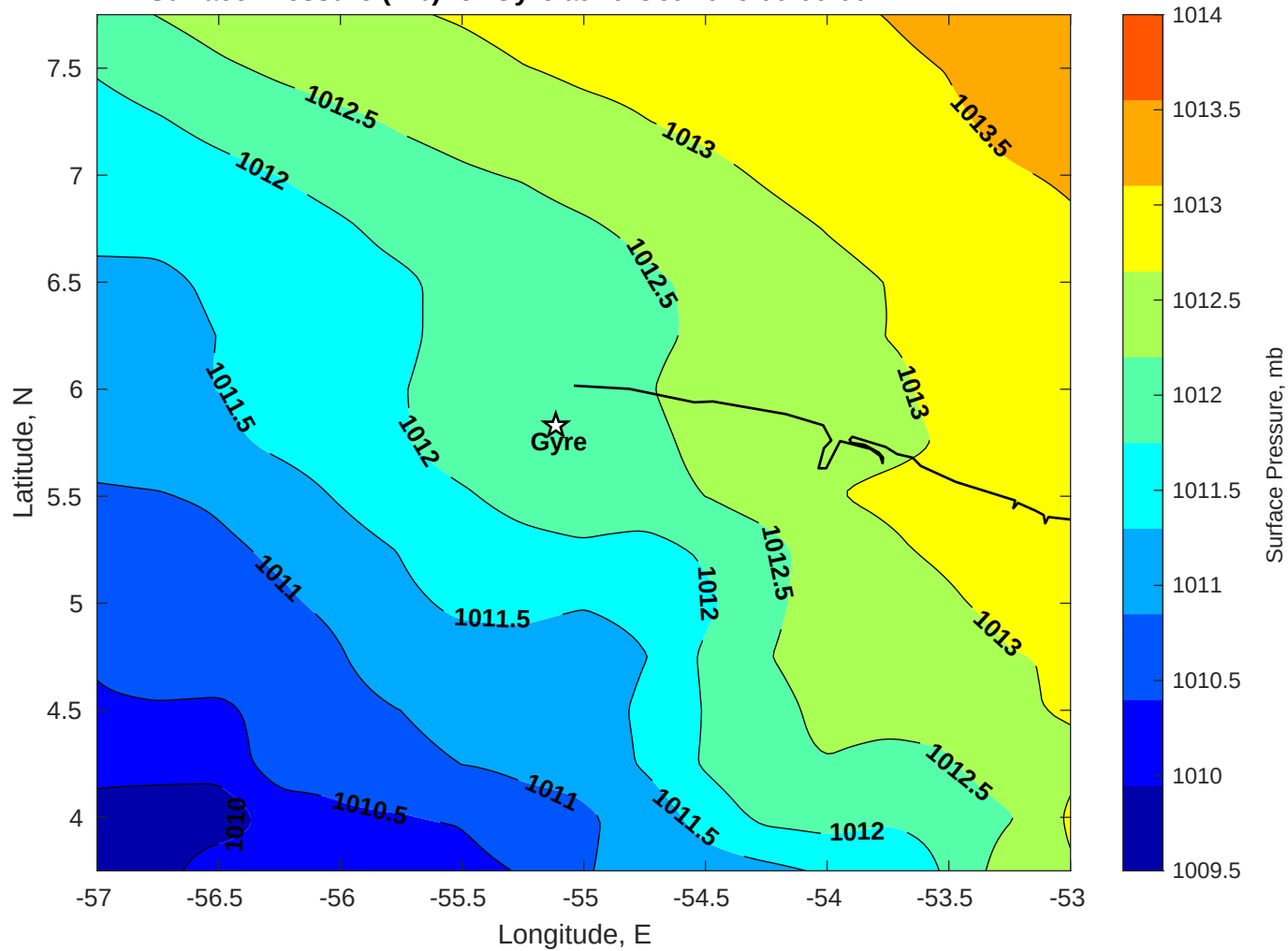
Surface Pressure (mb) for Gyre at 20-Oct-2025 00:00:00
