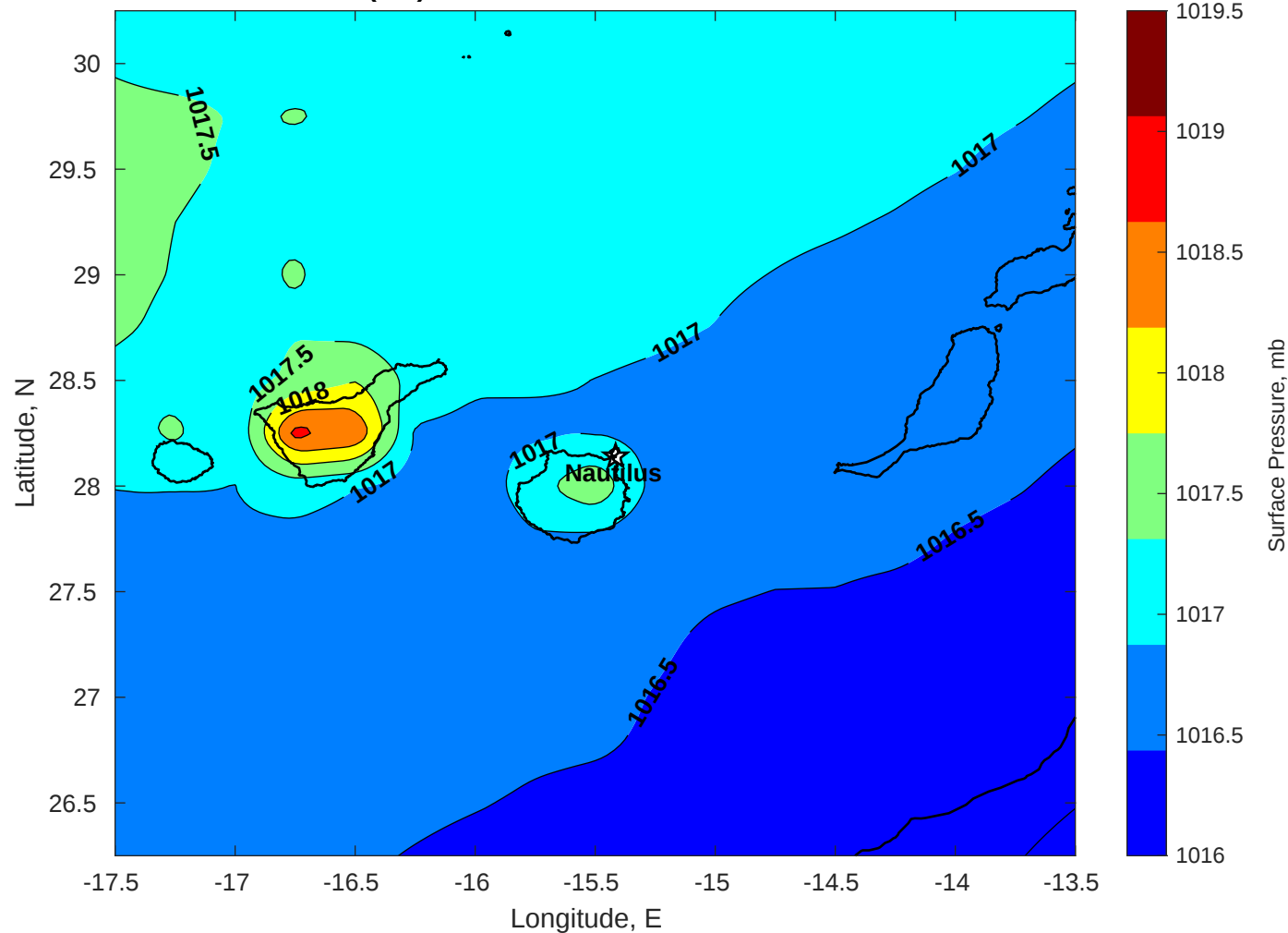
Surface Pressure (mb) for Nautilus at 19-Oct-2025 00:00:00
