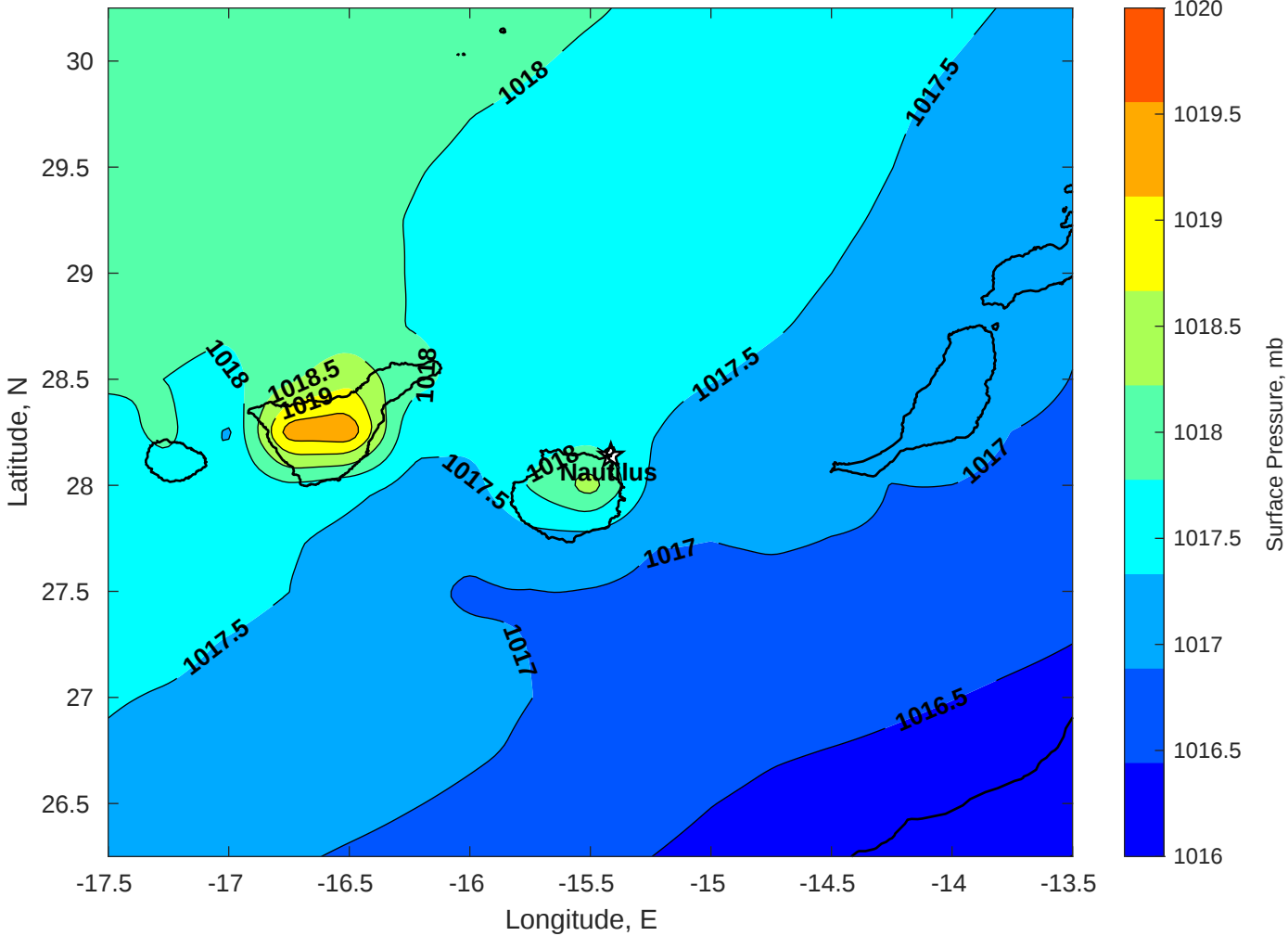
Surface Pressure (mb) for Nautilus at 21-Oct-2025 00:00:00
