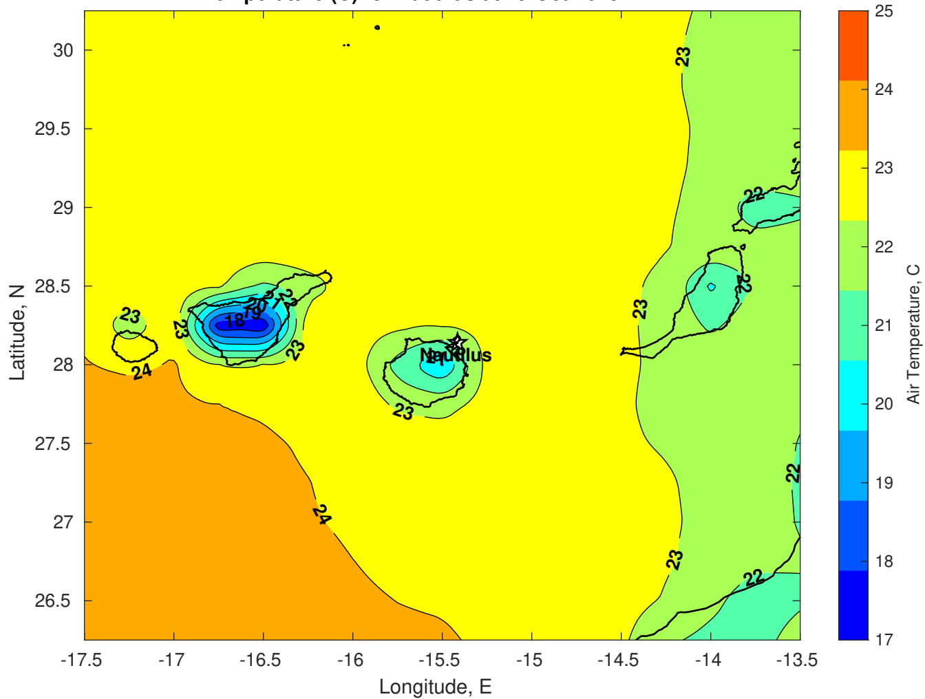
Air Temperature (C) for Nautilus at 19-Oct-2025
