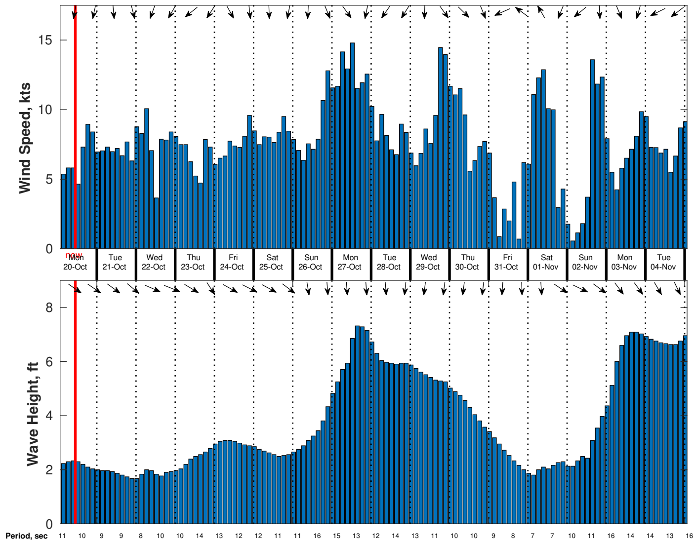
Wind & Wave Forecast for Nautilus from 19-Oct-2025 02:00:00 to 04-Nov-2025 02:00:00
