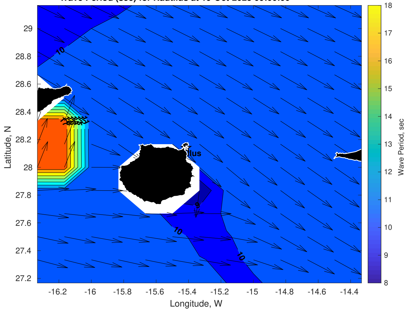
Wave Period (sec) for Nautilus at 19-Oct-2025 09:00:00
