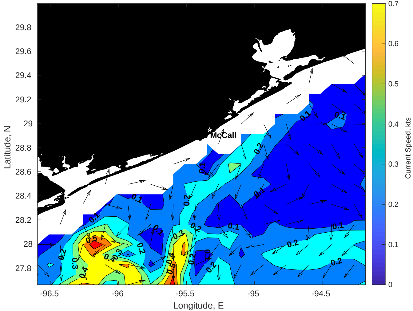
Surface Currents for Brooks McCall at 19-Oct-2025 00:00:00
