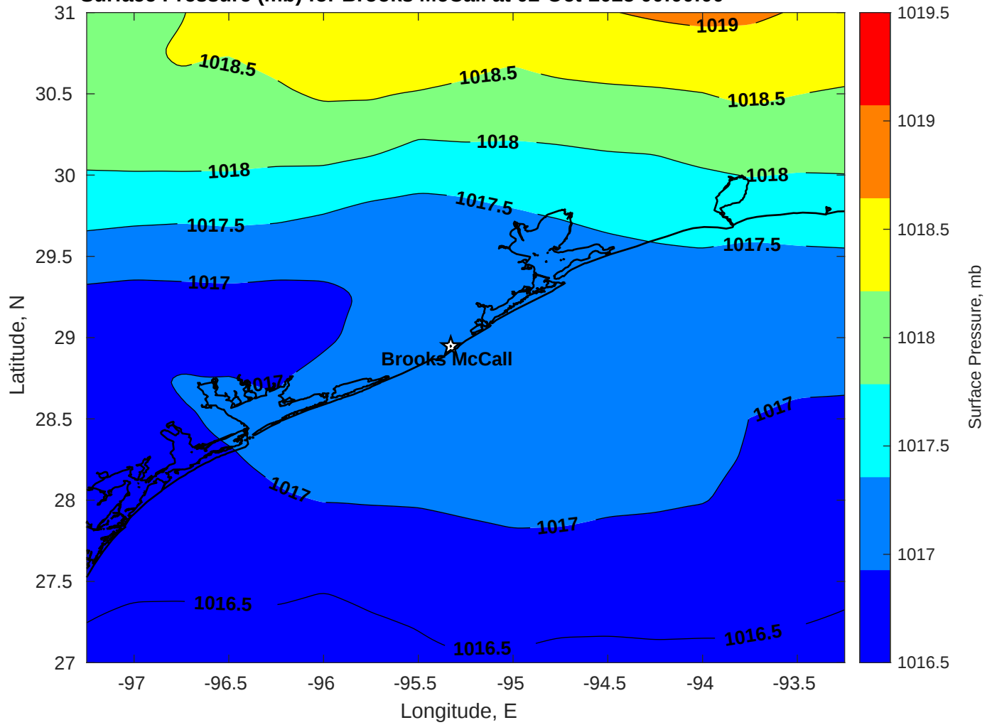
Surface Pressure (mb) for Brooks McCall at 02-Oct-2025 00:00:00
