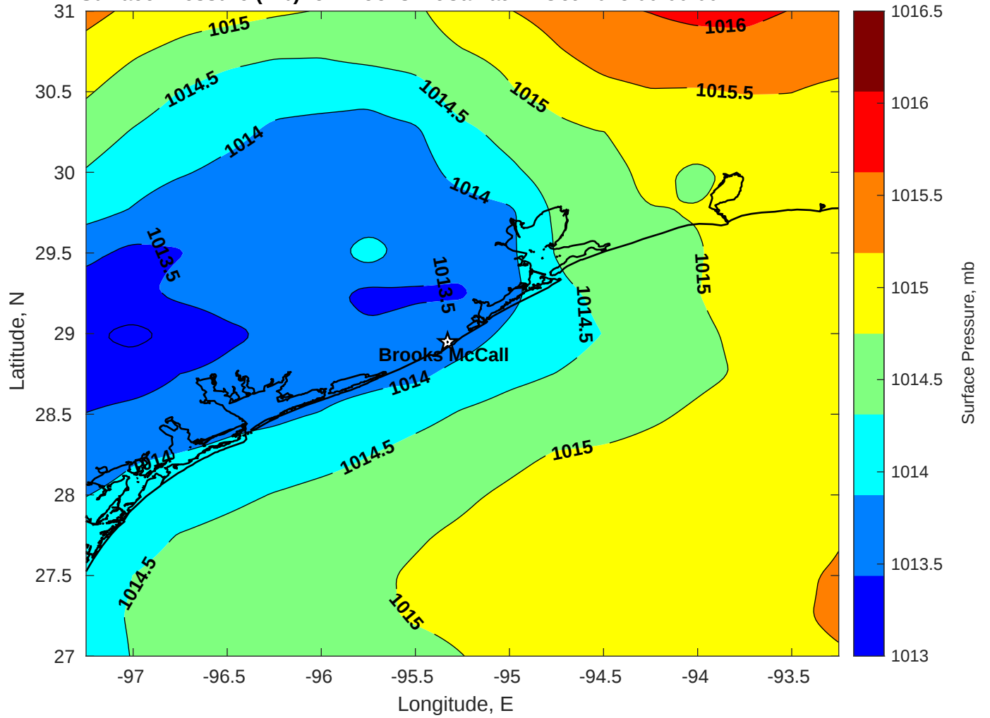
Surface Pressure (mb) for Brooks McCall at 22-Oct-2025 00:00:00
