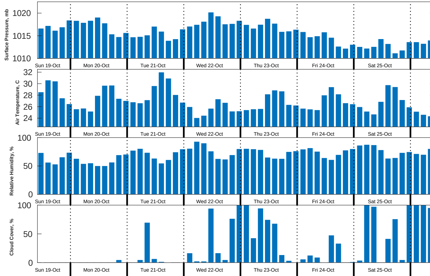
Met Forecast for Brooks McCall from 19-Oct-2025 12:00:00 to 26-Oct-2025 12:00:00
