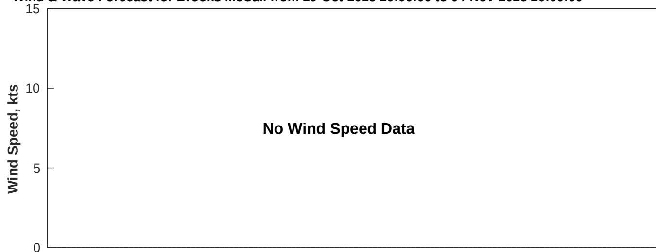
Wind & Wave Forecast for Brooks McCall from 19-Oct-2025 20:00:00 to 04-Nov-2025 20:00:00
