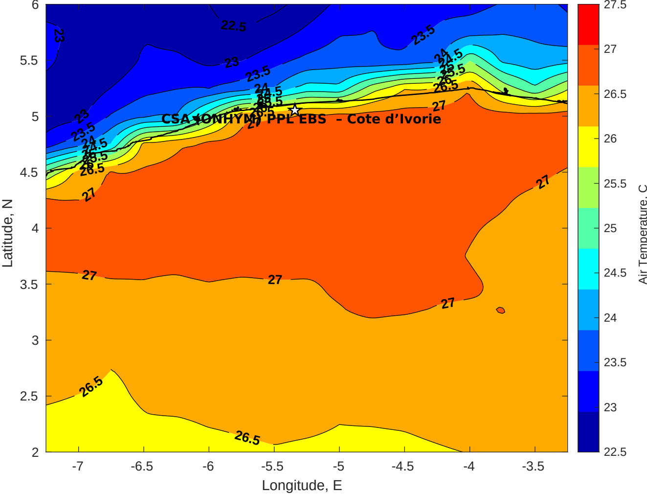
Air Temperature (C) for CSA (ONHYM) PPL EBS - Cote d'Ivoire at 20-Oct-2025
