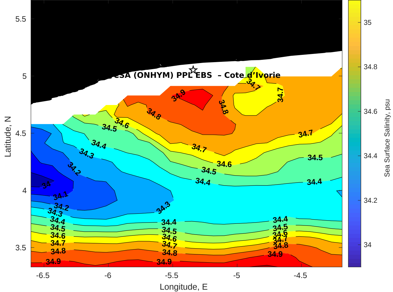
Surface Salinity for CSA (ONHYM) PPL EBS - Cote d'Ivoire at 19-Oct-2025 00:00:00
