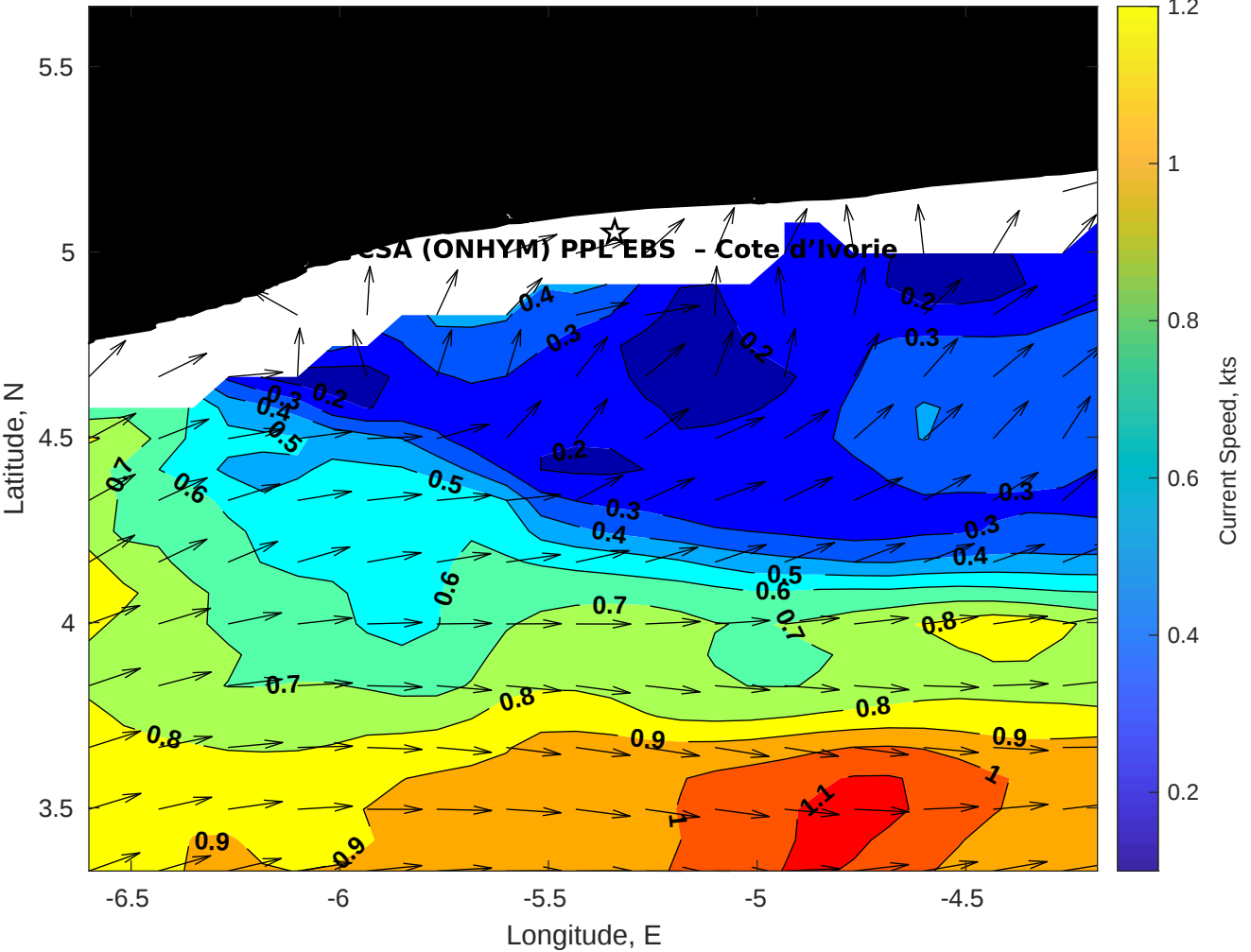
Surface Currents for CSA (ONHYM) PPL EBS - Cote d'Ivoire at 19-Oct-2025 00:00:00
