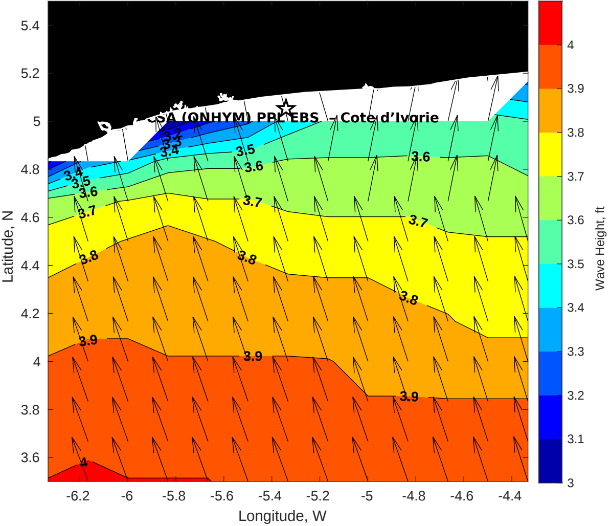
Wave Height (ft) for CSA (ONHYM) PPL EBS - Cote d'Ivoire at 20-Oct-2025 09:00:00
