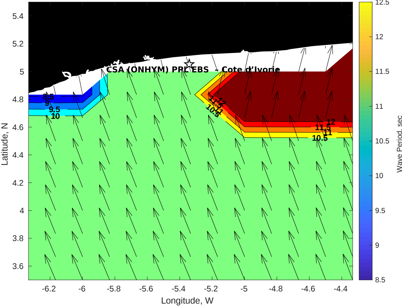
Wave Period (sec) for CSA (ONHYM) PPL EBS - Cote d'Ivoire at 20-Oct-2025 09:00:00
