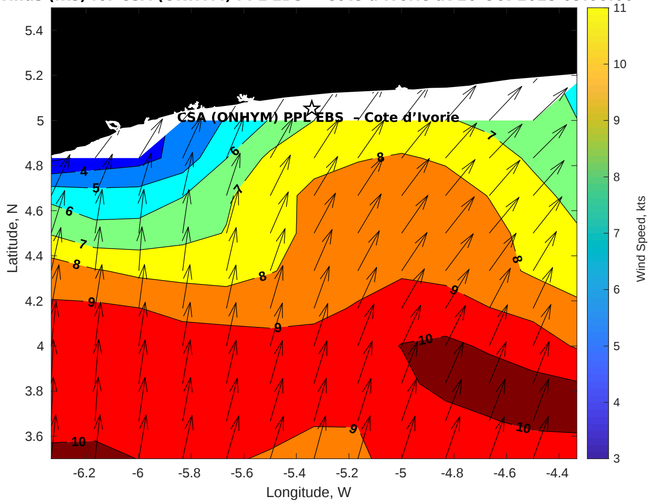
Winds (kts) for CSA (ONHYM) PPL EBS - Cote d'Ivoire at 20-Oct-2025 09:00:00
