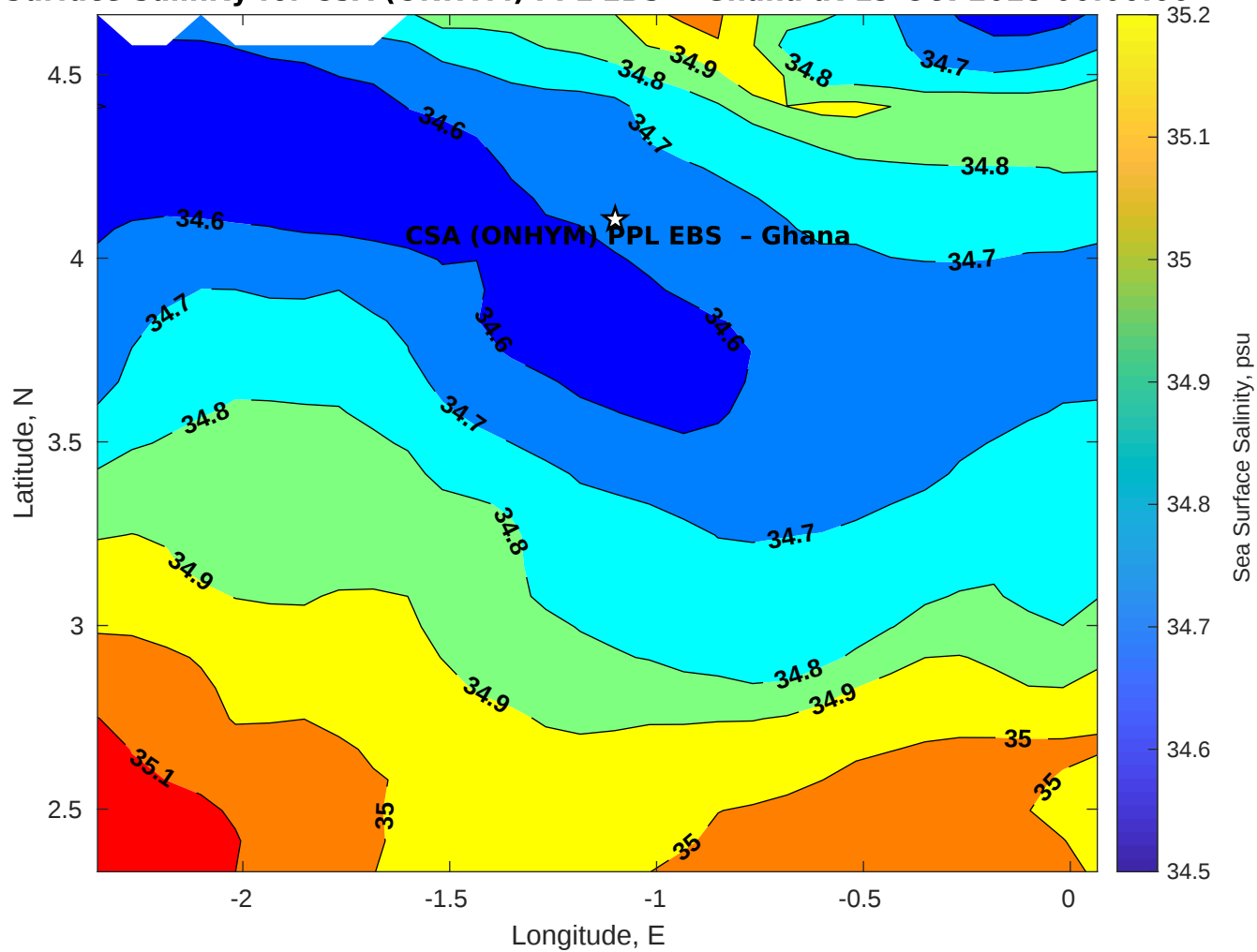
Surface Salinity for CSA (ONHYM) PPL EBS - Ghana at 19-Oct-2025 00:00:00
