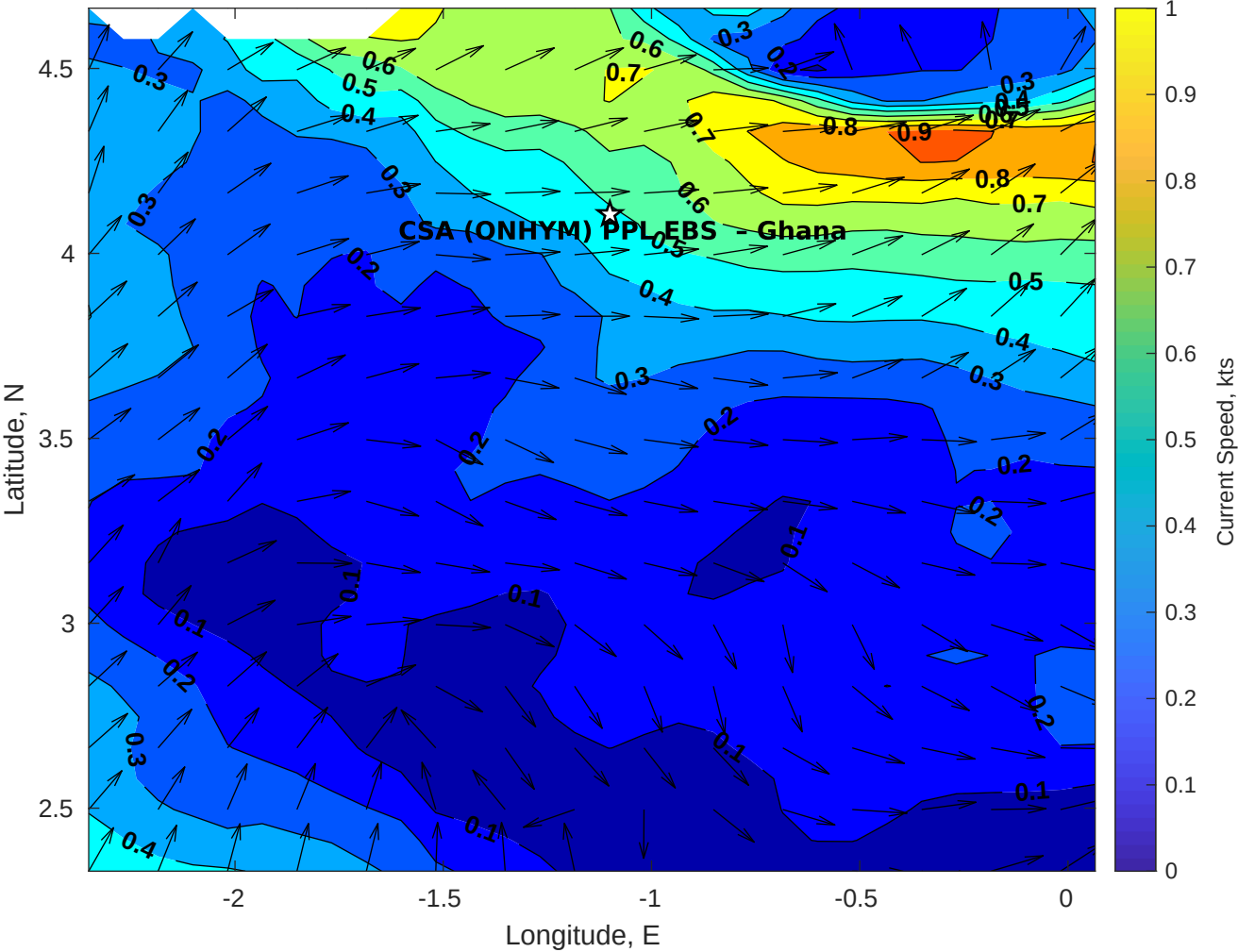
Surface Currents for CSA (ONHYM) PPL EBS - Ghana at 19-Oct-2025 00:00:00
