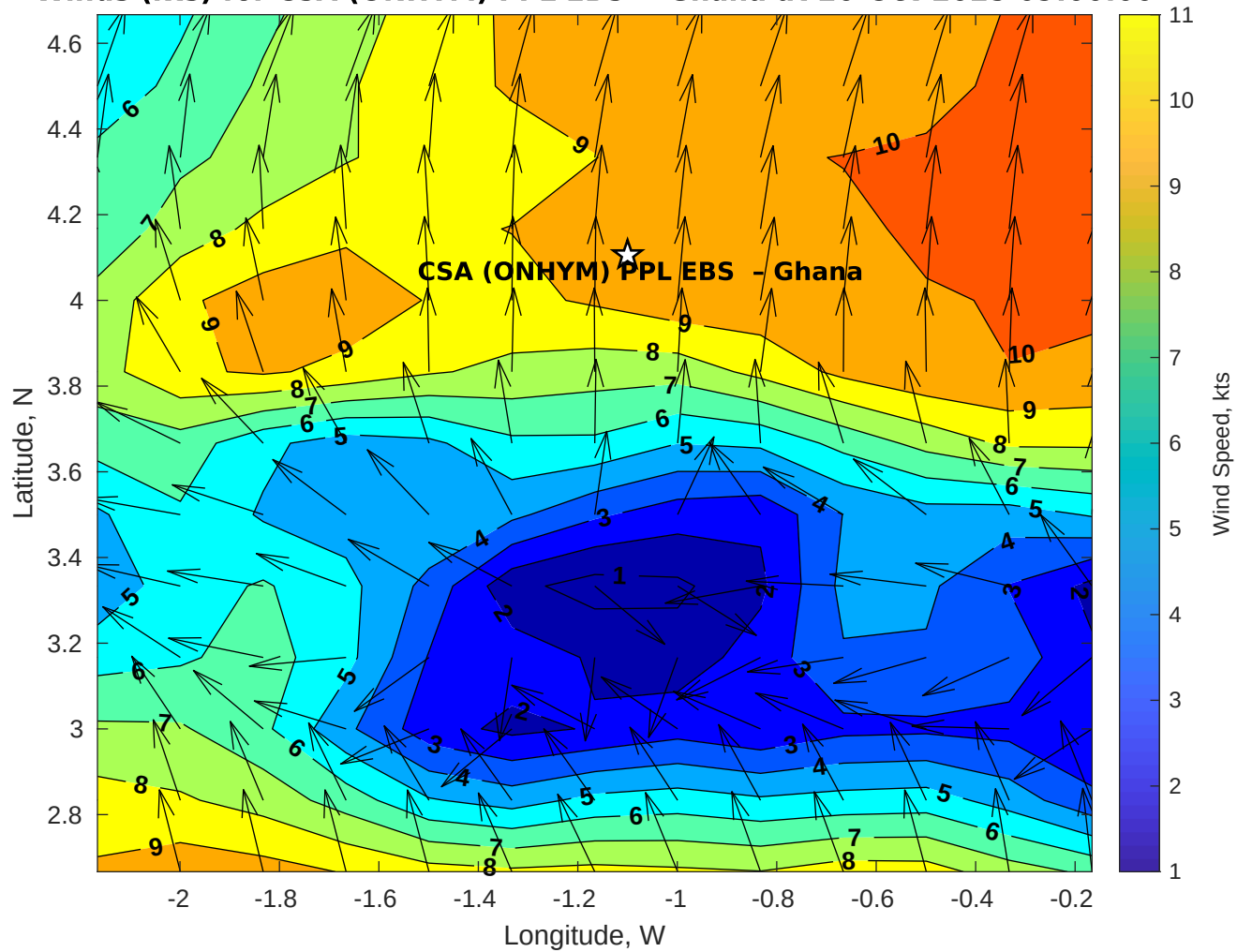
Winds (kts) for CSA (ONHYM) PPL EBS - Ghana at 20-Oct-2025 09:00:00
