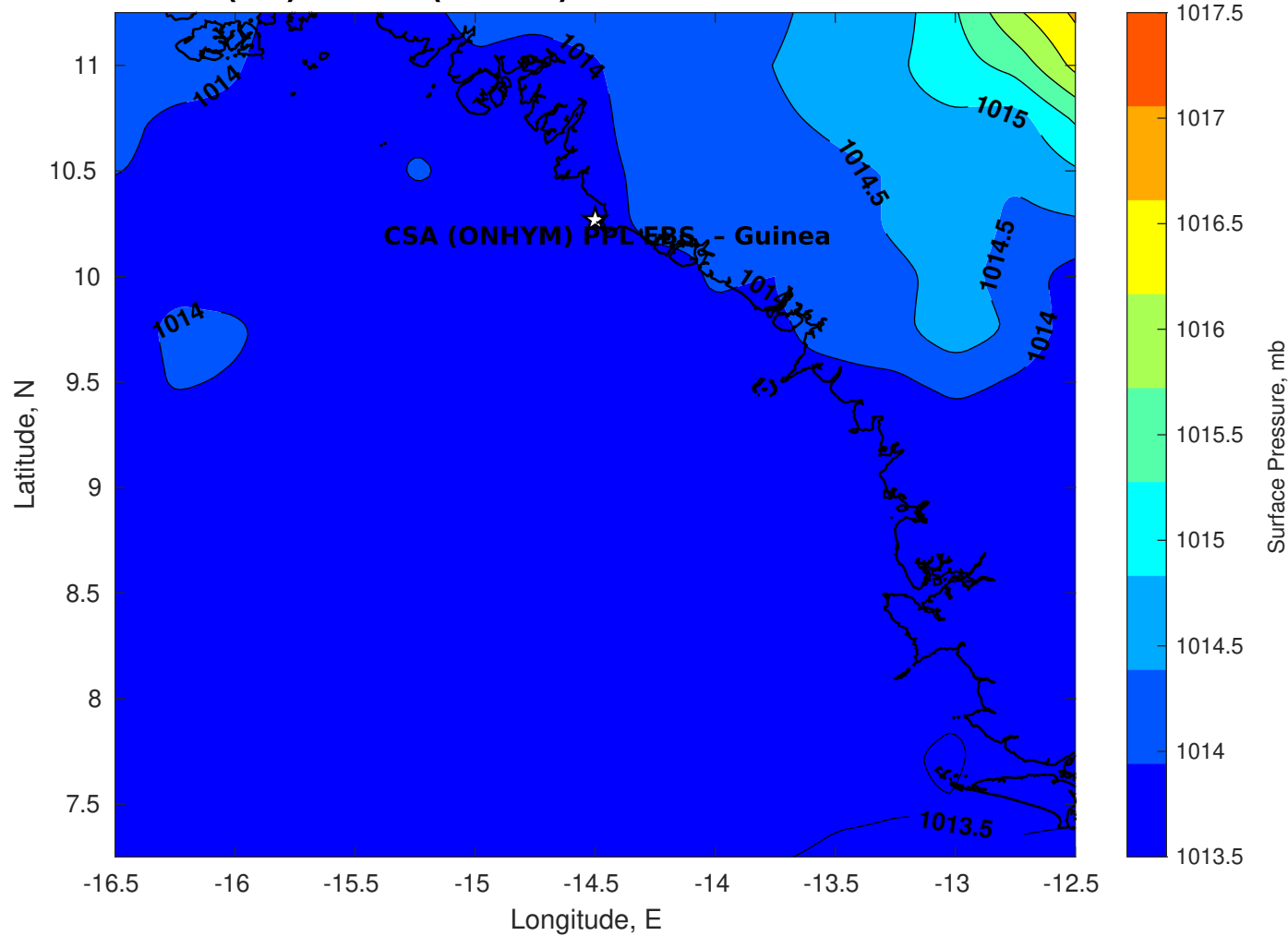
Surface Pressure (mb) for CSA (ONHYM) PPL EBS - Guinea at 20-Oct-2025 00:00:00
