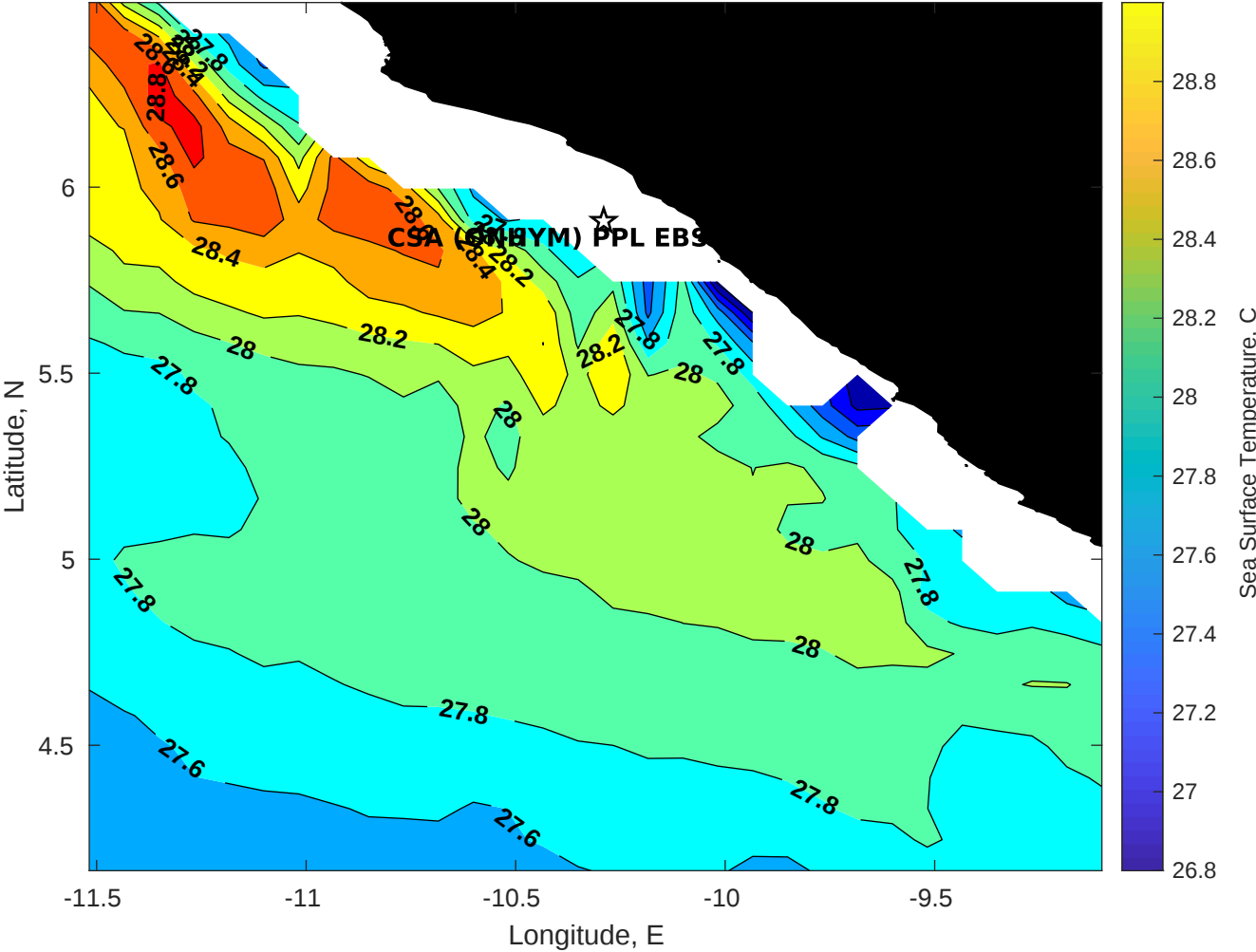
SST for CSA (ONHYM) PPL EBS - Liberia at 19-Oct-2025 00:00:00
