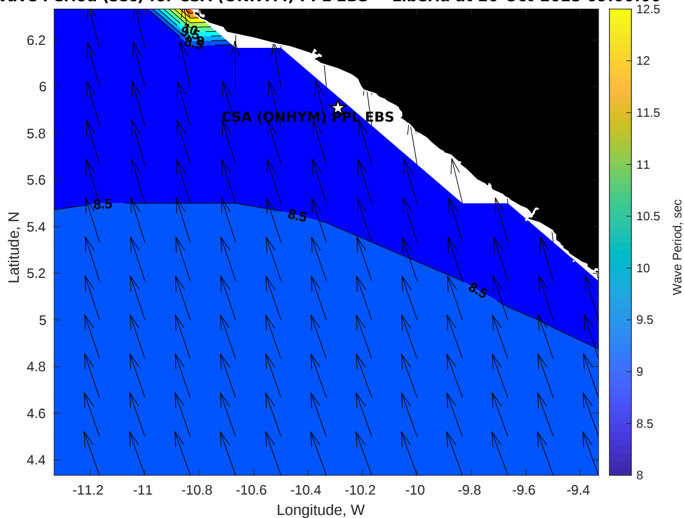
Wave Period (sec) for CSA (ONHYM) PPL EBS - Liberia at 20-Oct-2025 09:00:00
