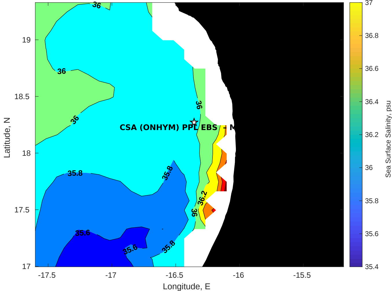
Surface Salinity for CSA (ONHYM) PPL EBS - Mauritania at 19-Oct-2025 00:00:00
