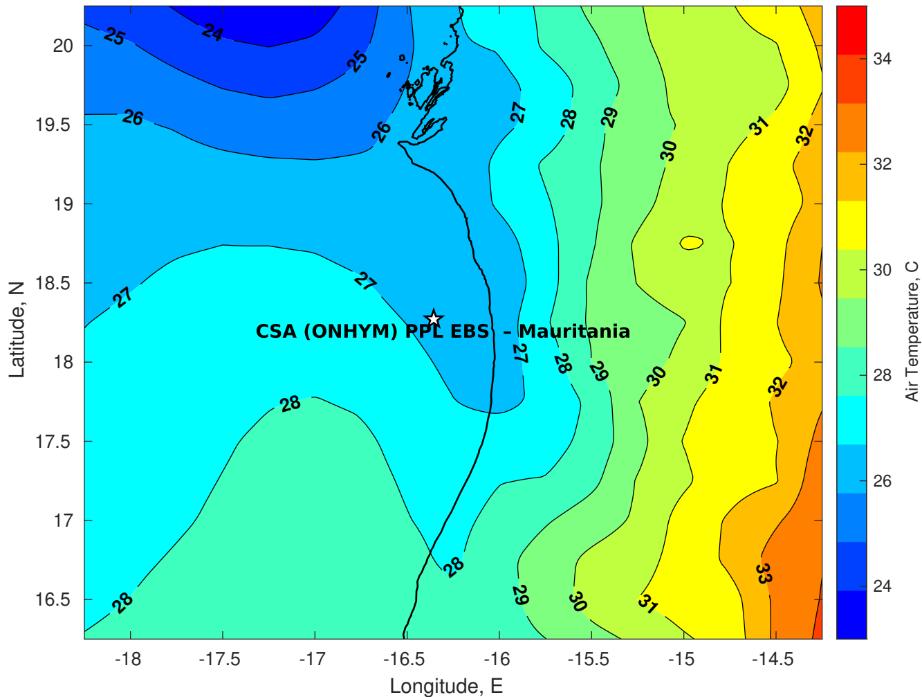
Air Temperature (C) for CSA (ONHYM) PPL EBS - Mauritania at 20-Oct-2025
