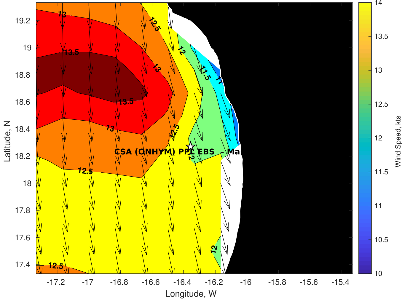
Winds (kts) for CSA (ONHYM) PPL EBS - Mauritania at 20-Oct-2025 09:00:00
