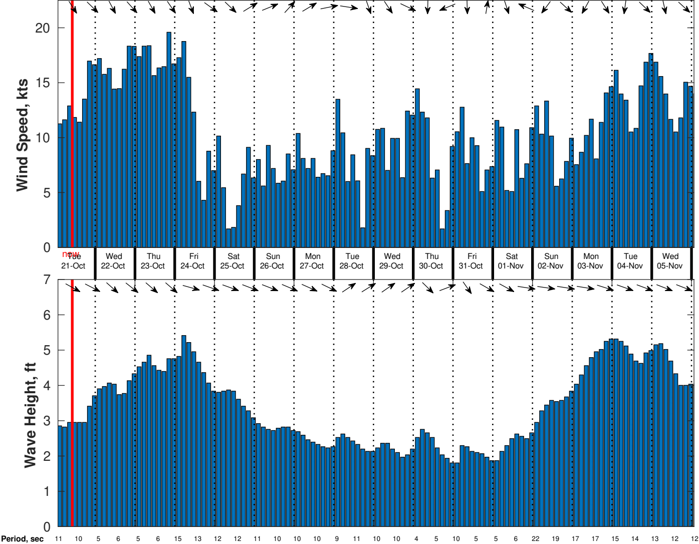
Wind & Wave Forecast for CSA (ONHYM) PPL EBS - Mauritania from 20-Oct-2025 01:00:00 to 05-Nov-2025 01:00:00
