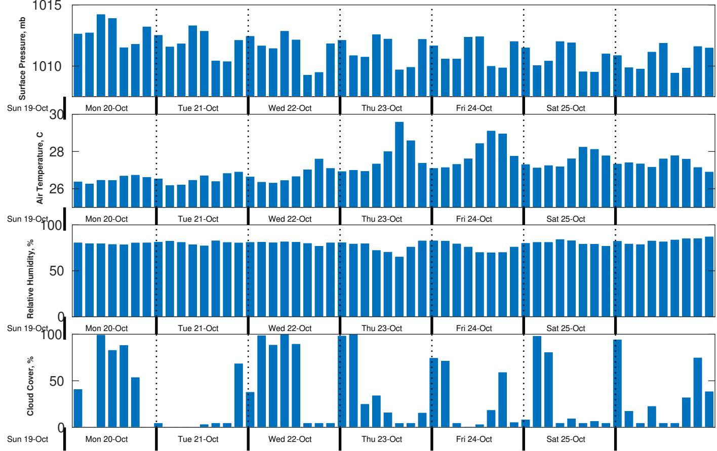
Met Forecast for CSA (ONHYM) PPL EBS - Mauritania from 20-Oct-2025 00:00:00 to 27-Oct-2025 00:00:00
