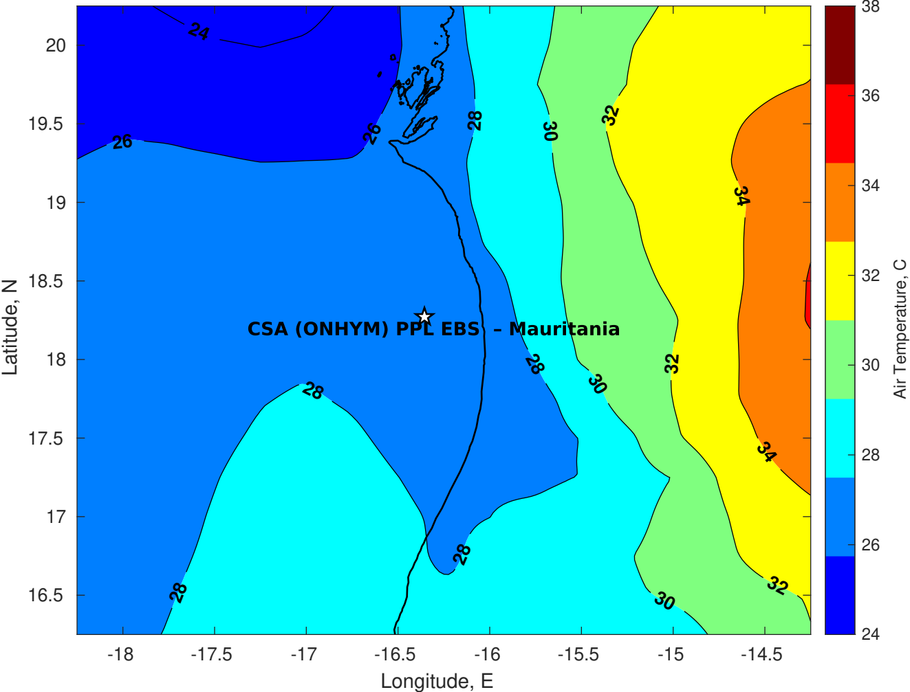
Air Temperature (C) for CSA (ONHYM) PPL EBS - Mauritania at 20-Oct-2025
