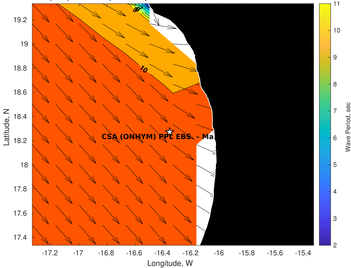
Wave Period (sec) for CSA (ONHYM) PPL EBS - Mauritania at 20-Oct-2025 09:00:00
