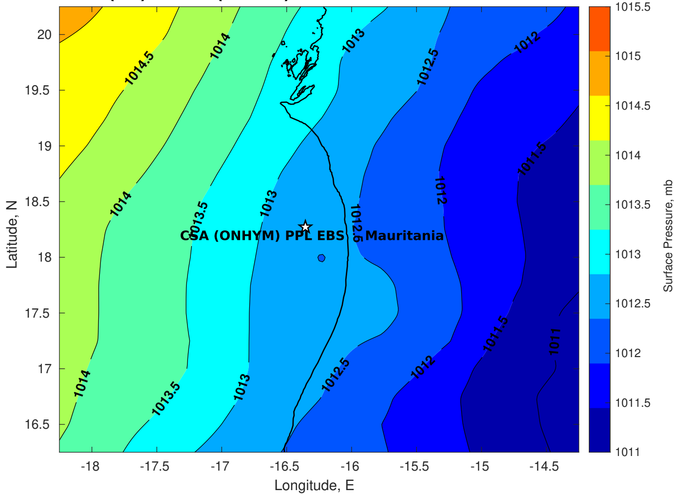
Surface Pressure (mb) for CSA (ONHYM) PPL EBS - Mauritania at 21-Oct-2025 00:00:00
