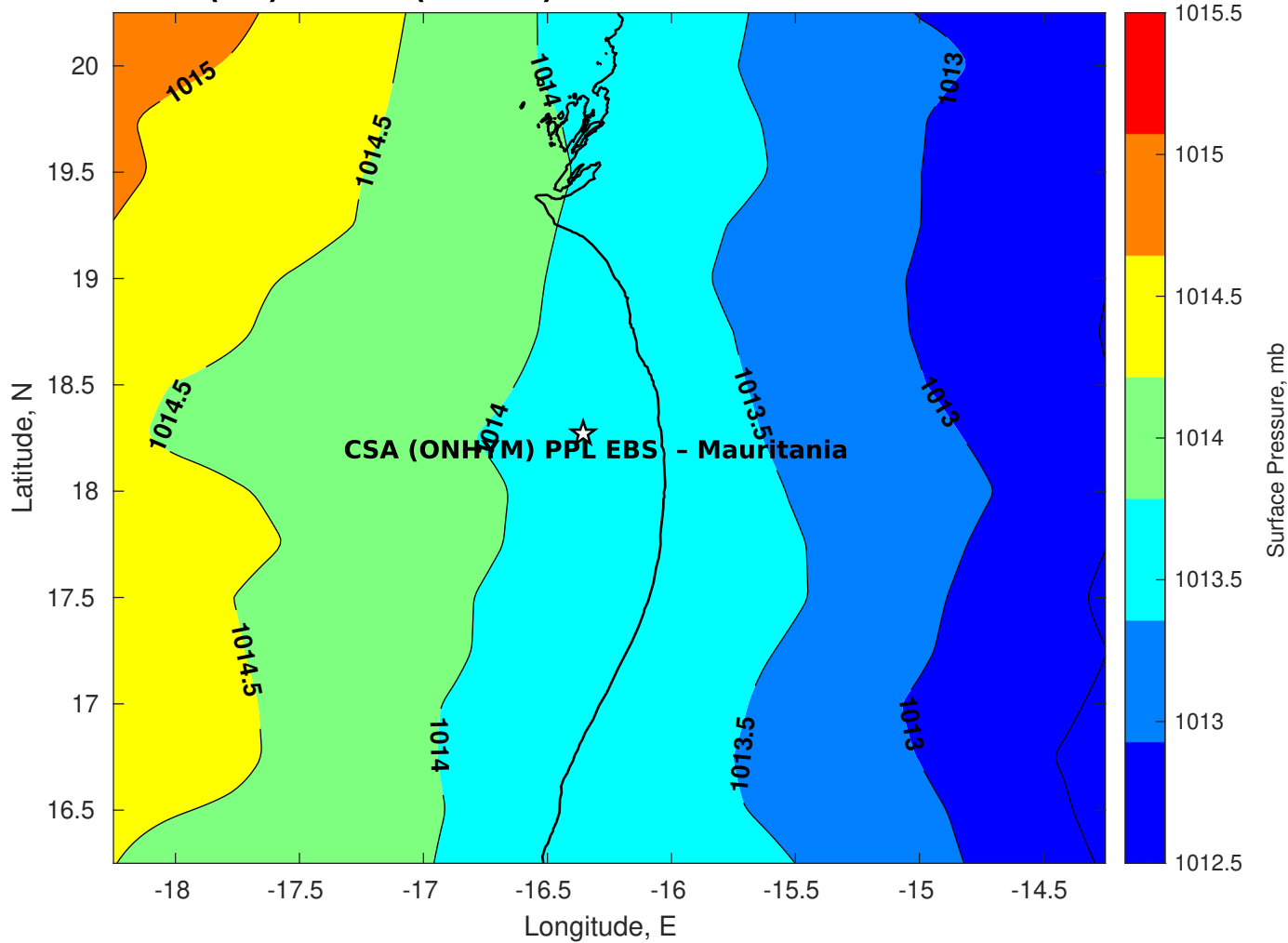
Surface Pressure (mb) for CSA (ONHYM) PPL EBS - Mauritania at 20-Oct-2025 00:00:00
