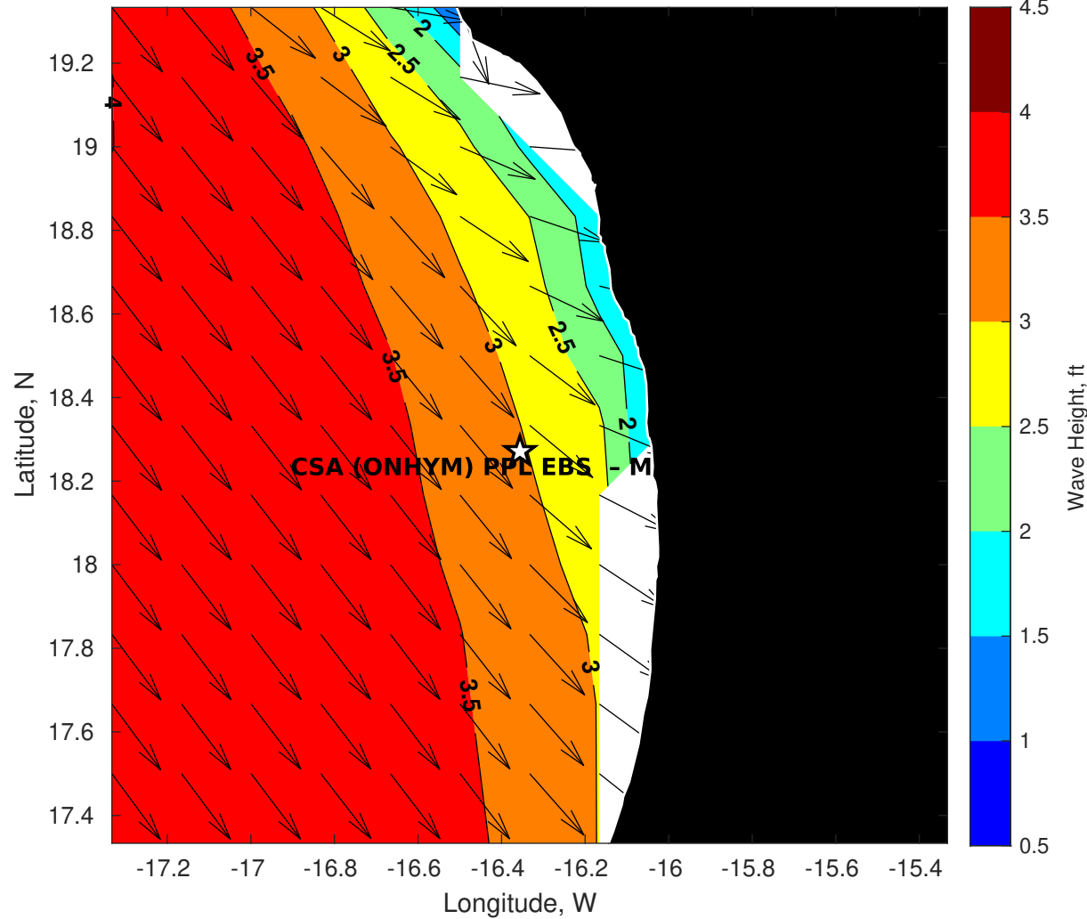
Wave Height (ft) for CSA (ONHYM) PPL EBS - Mauritania at 20-Oct-2025 09:00:00
