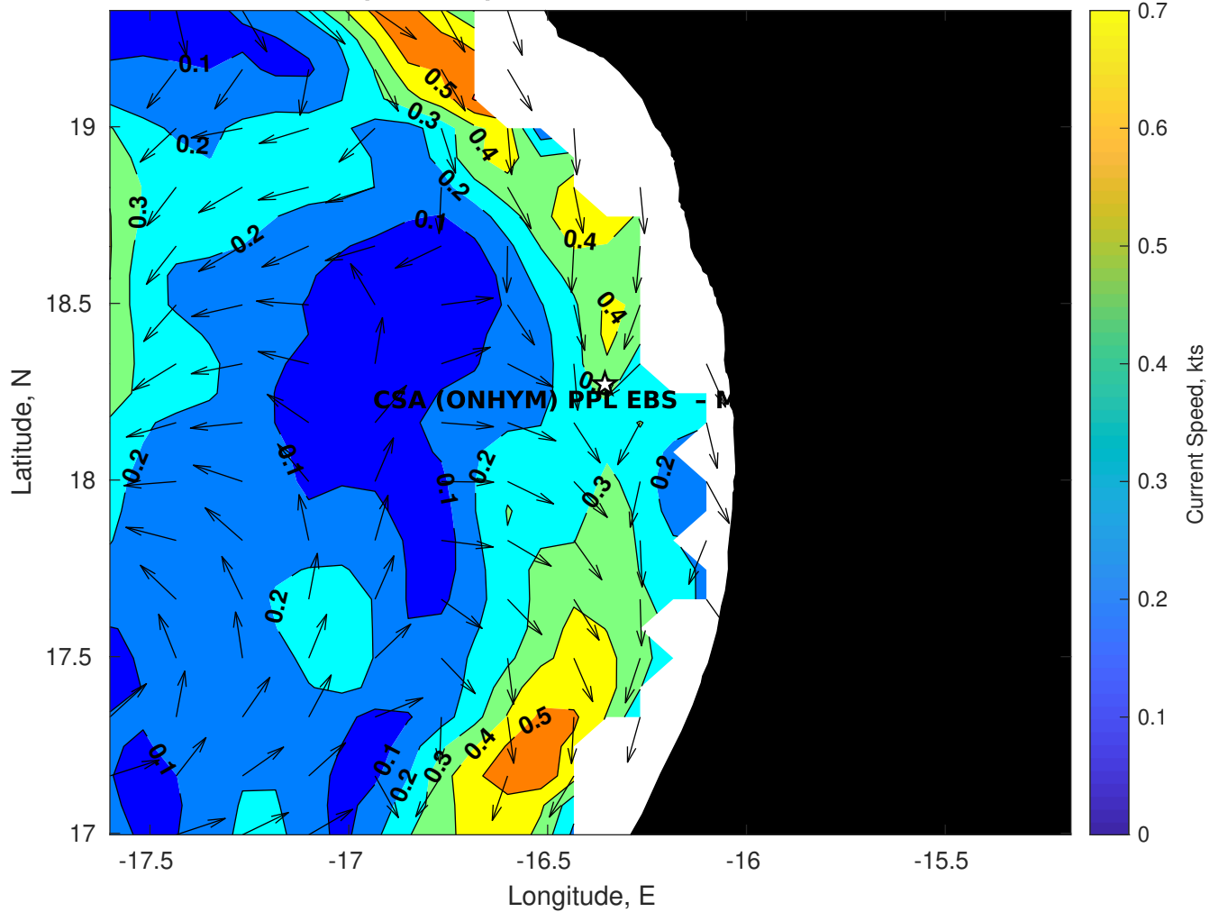
Surface Currents for CSA (ONHYM) PPL EBS - Mauritania at 19-Oct-2025 00:00:00
