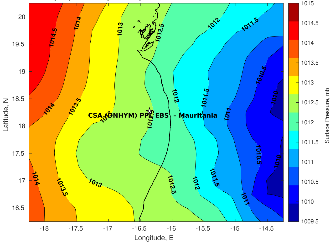
Surface Pressure (mb) for CSA (ONHYM) PPL EBS - Mauritania at 22-Oct-2025 00:00:00
