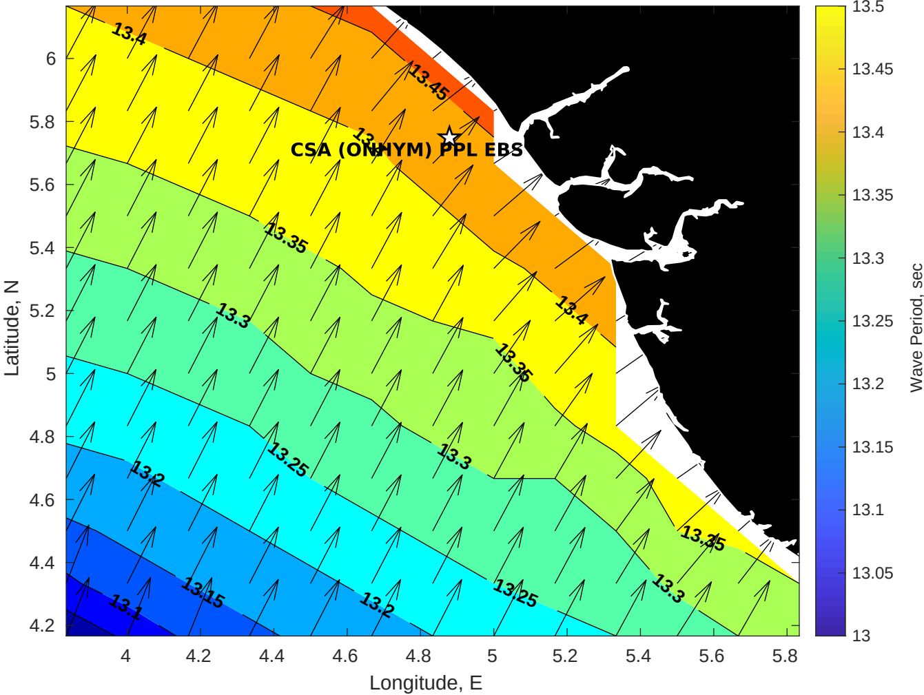
Wave Period (sec) for CSA (ONHYM) PPL EBS - Nigeria at 20-Oct-2025 09:00:00
