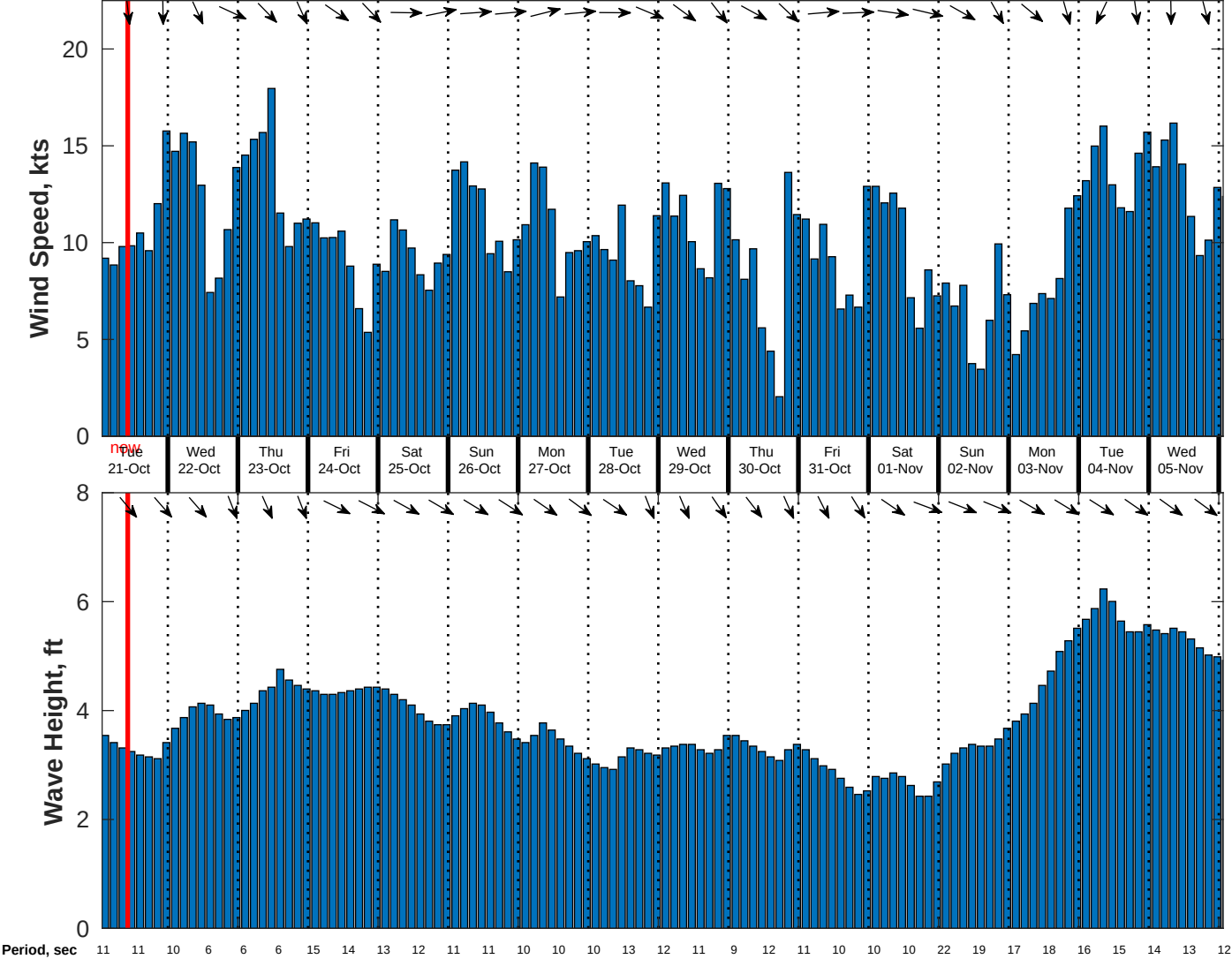
Wind & Wave Forecast for CSA (ONHYM) PPL EBS - Senegal from 20-Oct-2025 01:00:00 to 05-Nov-2025 01:00:00
