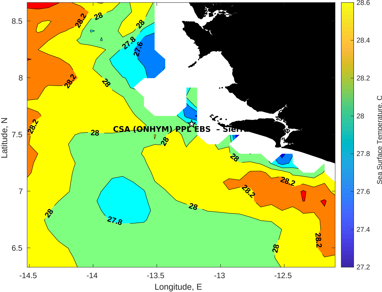
SST for CSA (ONHYM) PPL EBS - Sierra Leone at 19-Oct-2025 00:00:00
