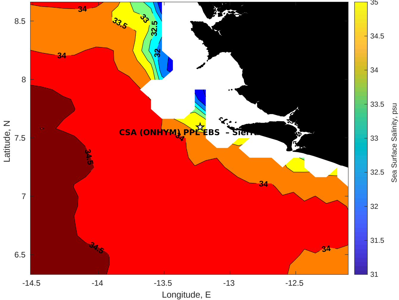
Surface Salinity for CSA (ONHYM) PPL EBS - Sierra Leone at 19-Oct-2025 00:00:00
