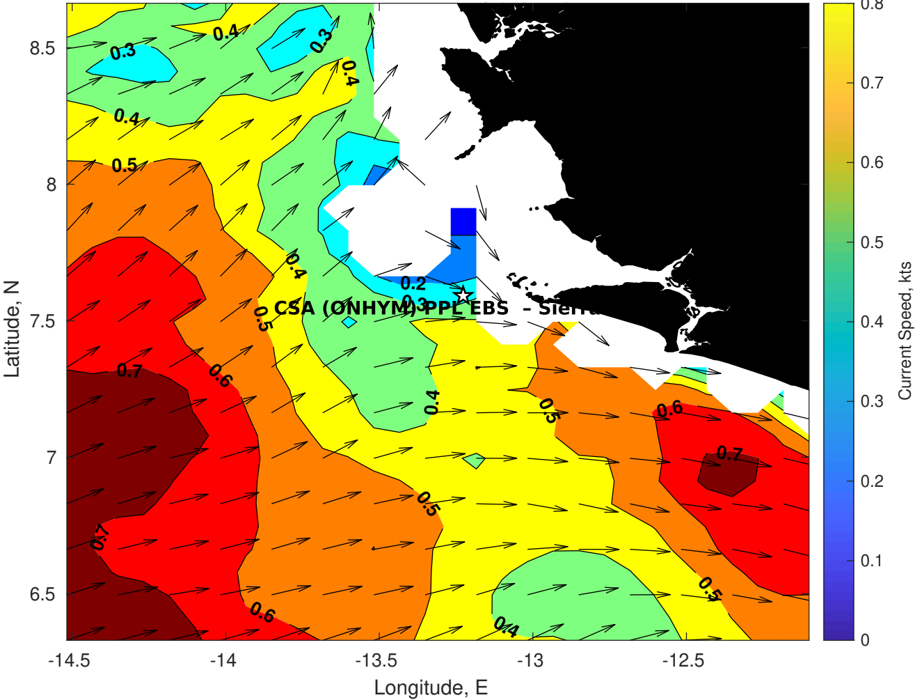
Surface Currents for CSA (ONHYM) PPL EBS - Sierra Leone at 19-Oct-2025 00:00:00
