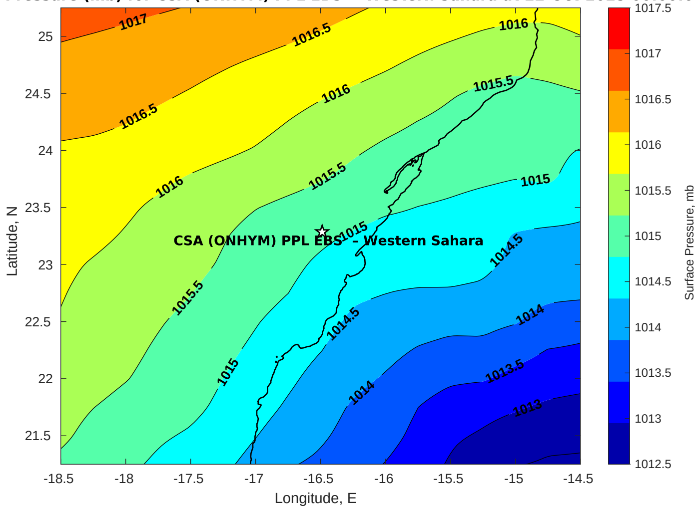
Surface Pressure (mb) for CSA (ONHYM) PPL EBS - Western Sahara at 22-Oct-2025 00:00:00
