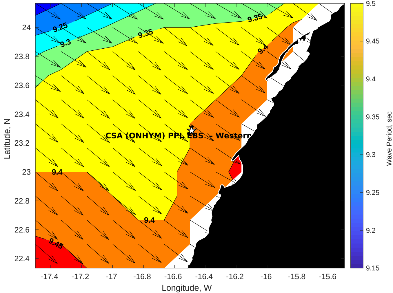
Wave Period (sec) for CSA (ONHYM) PPL EBS - Western Sahara at 20-Oct-2025 09:00:00
