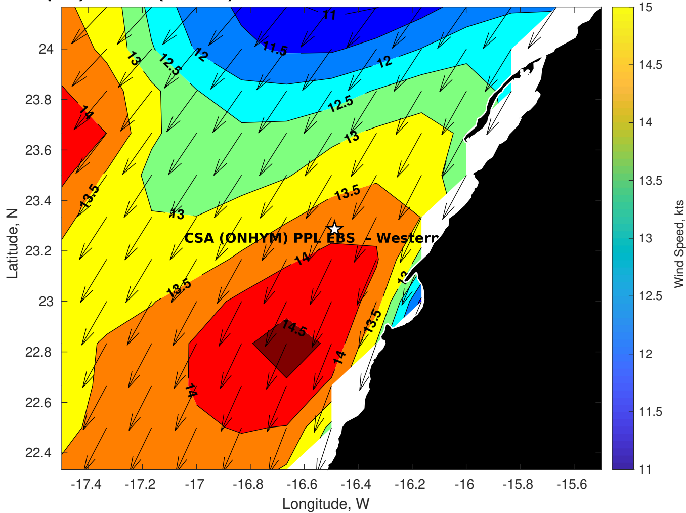
Winds (kts) for CSA (ONHYM) PPL EBS - Western Sahara at 20-Oct-2025 09:00:00
