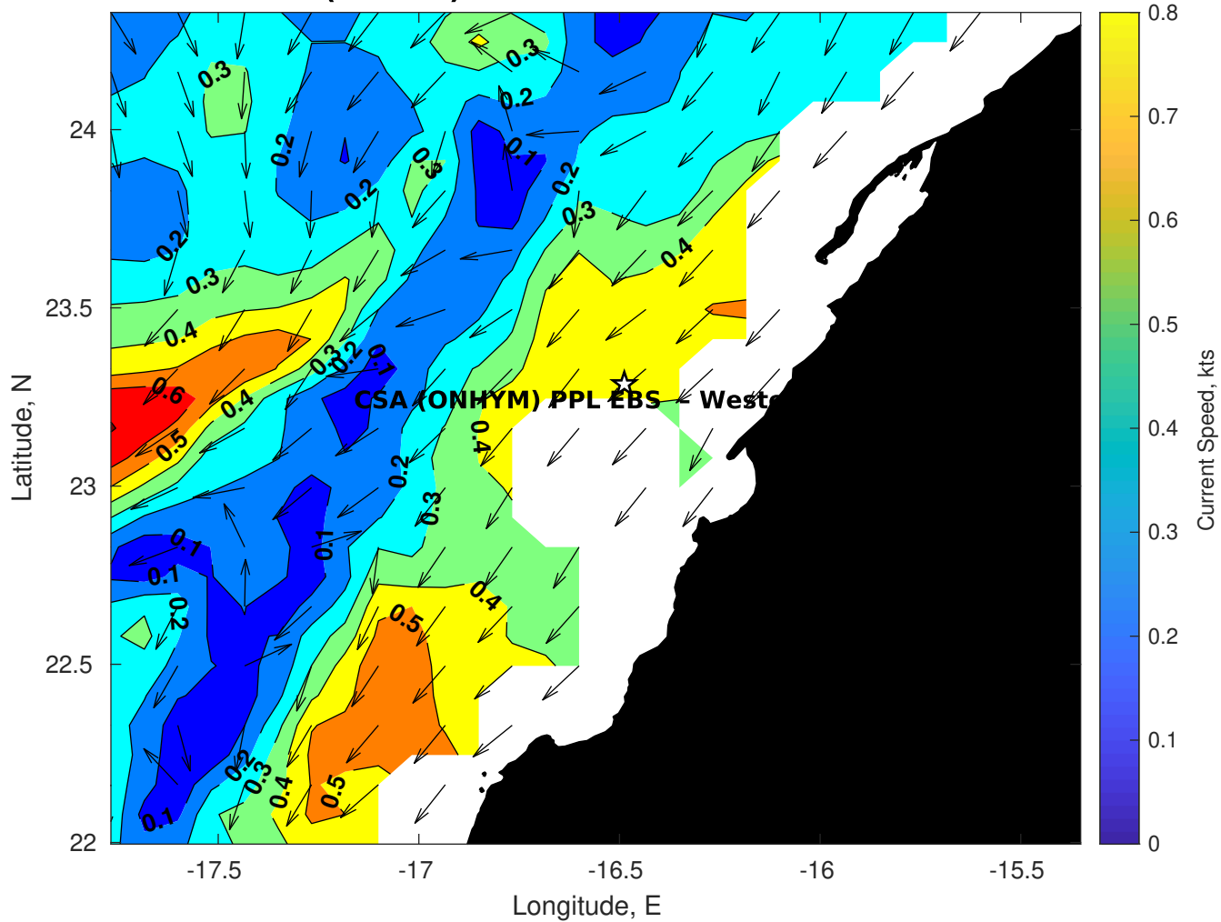
Surface Currents for CSA (ONHYM) PPL EBS - Western Sahara at 19-Oct-2025 00:00:00
