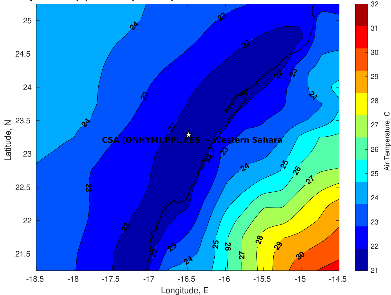
Air Temperature (C) for CSA (ONHYM) PPL EBS - Western Sahara at 20-Oct-2025
