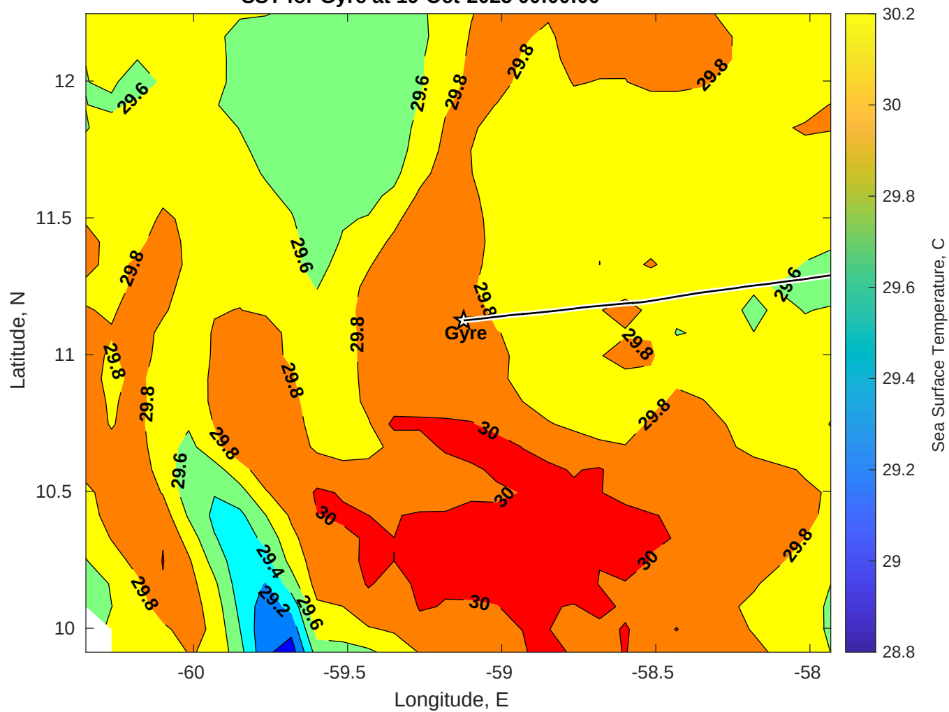
SST for Gyre at 19-Oct-2025 00:00:00
