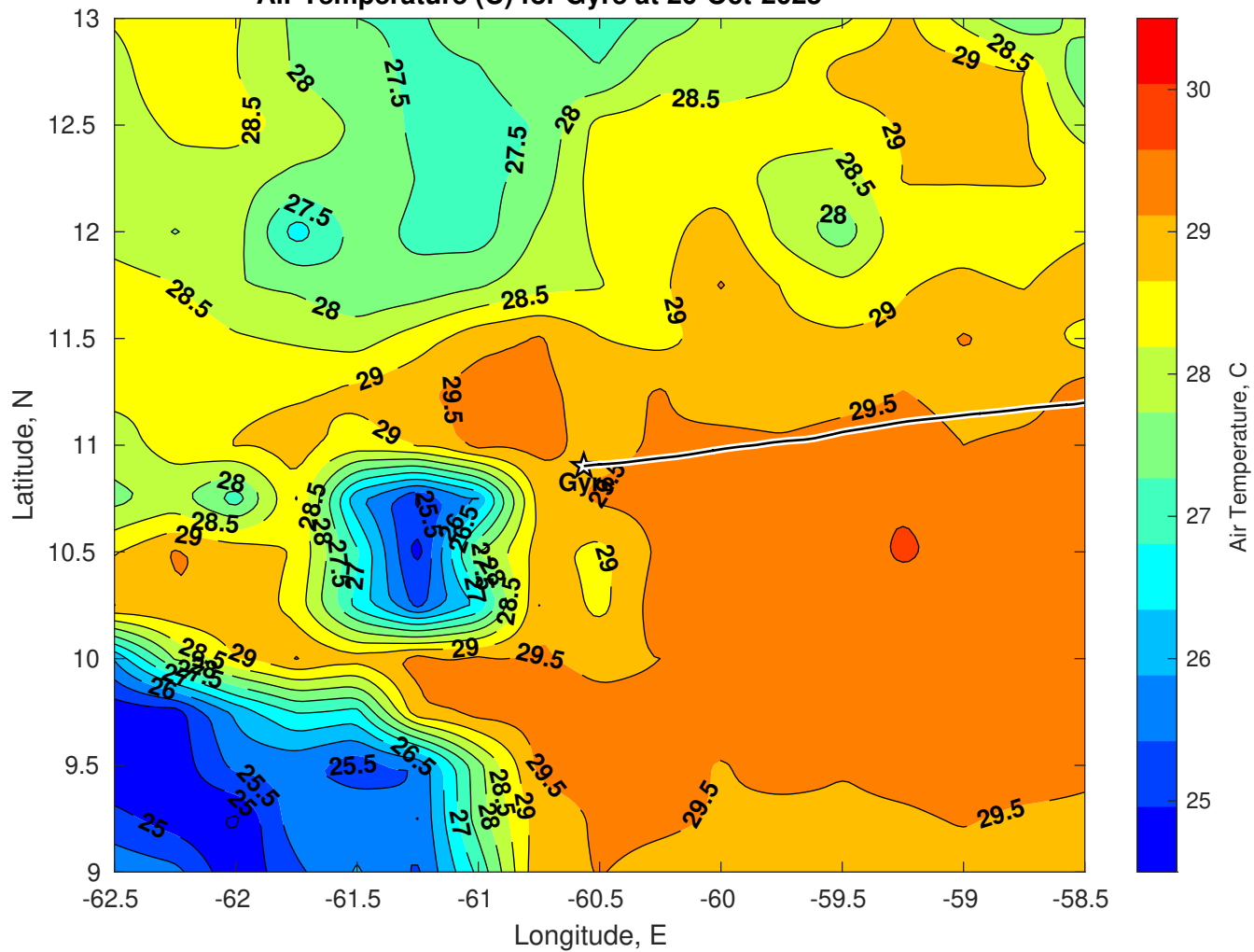
Air Temperature (C) for Gyre at 20-Oct-2025
