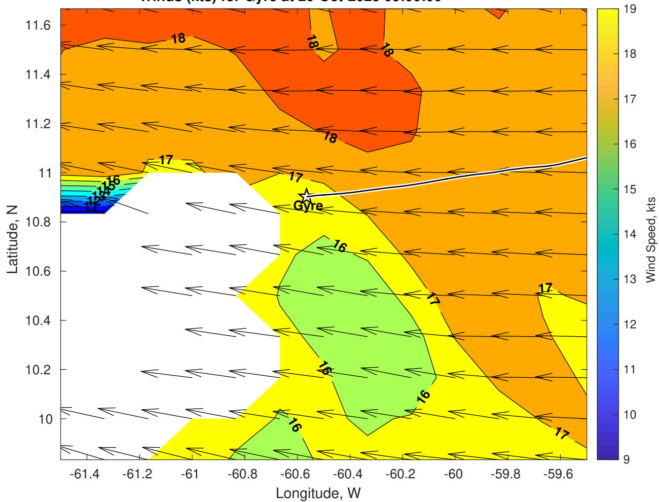
Winds (kts) for Gyre at 20-Oct-2025 09:00:00
