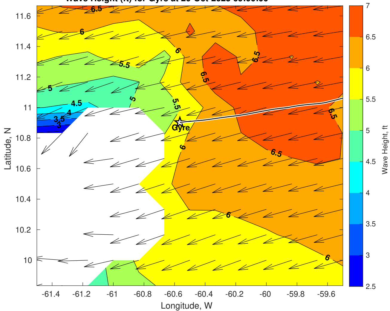
Wave Height (ft) for Gyre at 20-Oct-2025 09:00:00
