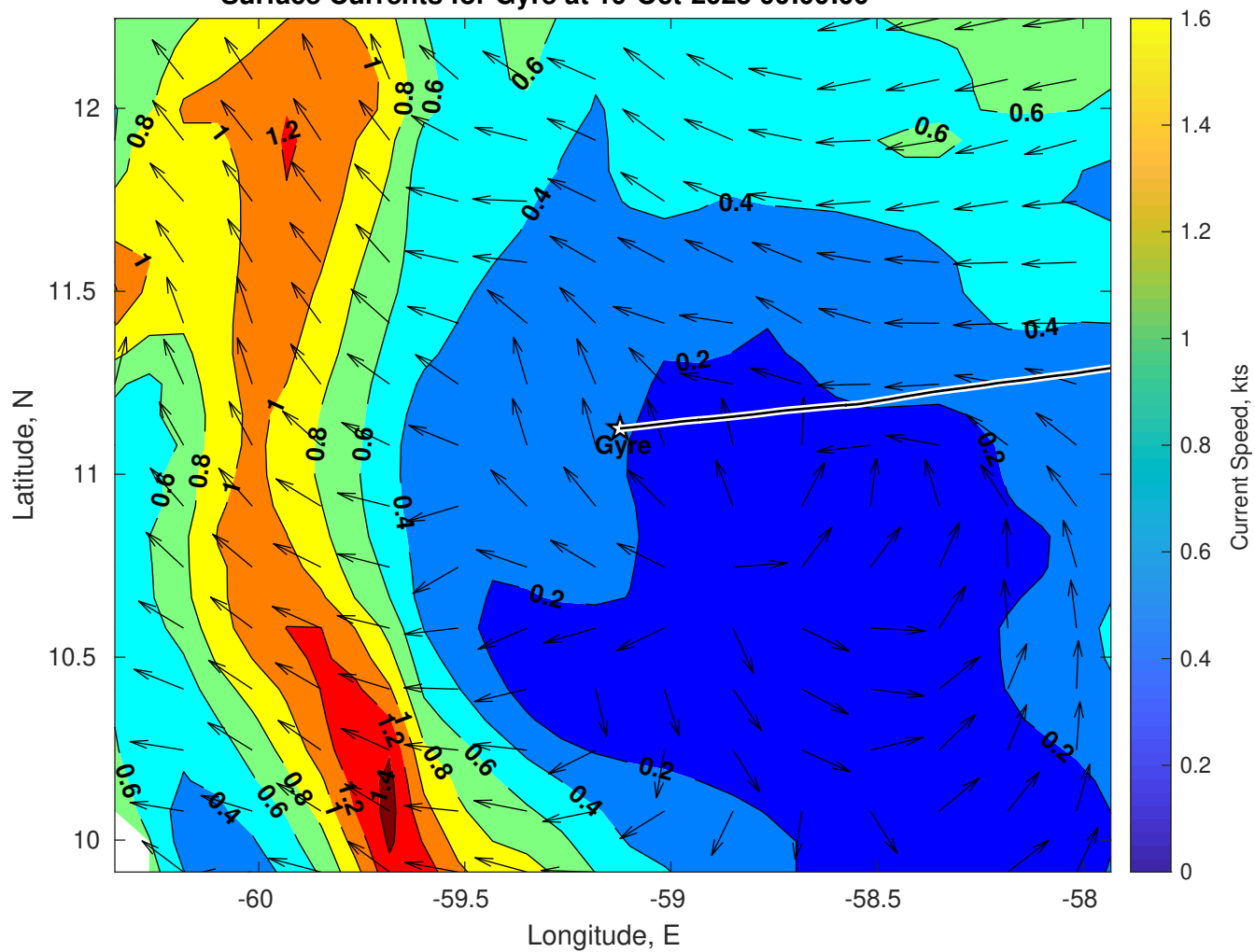
Surface Currents for Gyre at 19-Oct-2025 00:00:00
