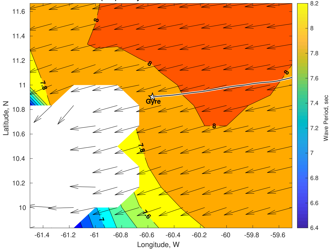
Wave Period (sec) for Gyre at 20-Oct-2025 09:00:00
