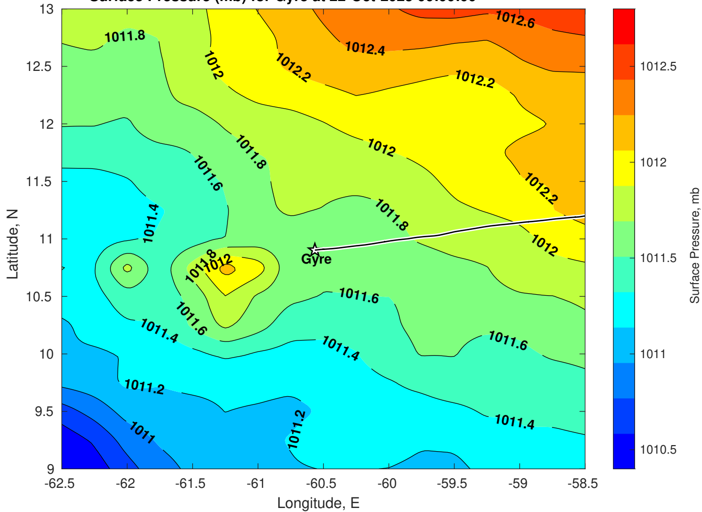
Surface Pressure (mb) for Gyre at 22-Oct-2025 00:00:00
