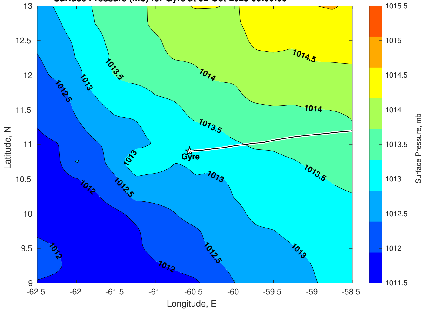
Surface Pressure (mb) for Gyre at 02-Oct-2025 00:00:00
