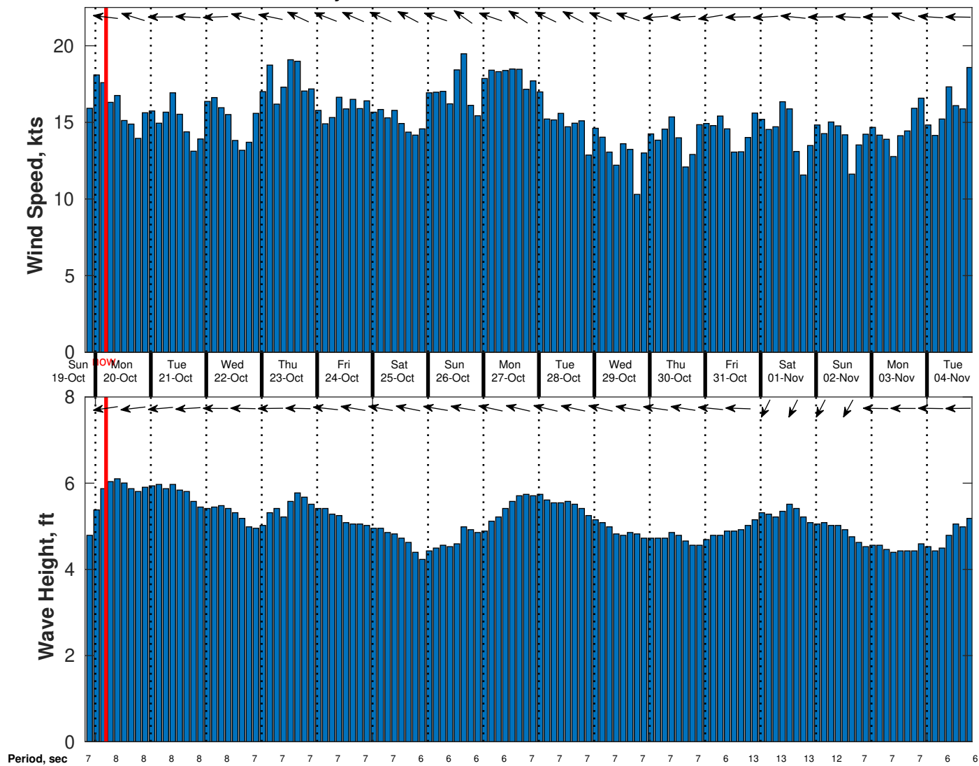
Wind & Wave Forecast for Gyre from 19-Oct-2025 20:00:00 to 04-Nov-2025 20:00:00
