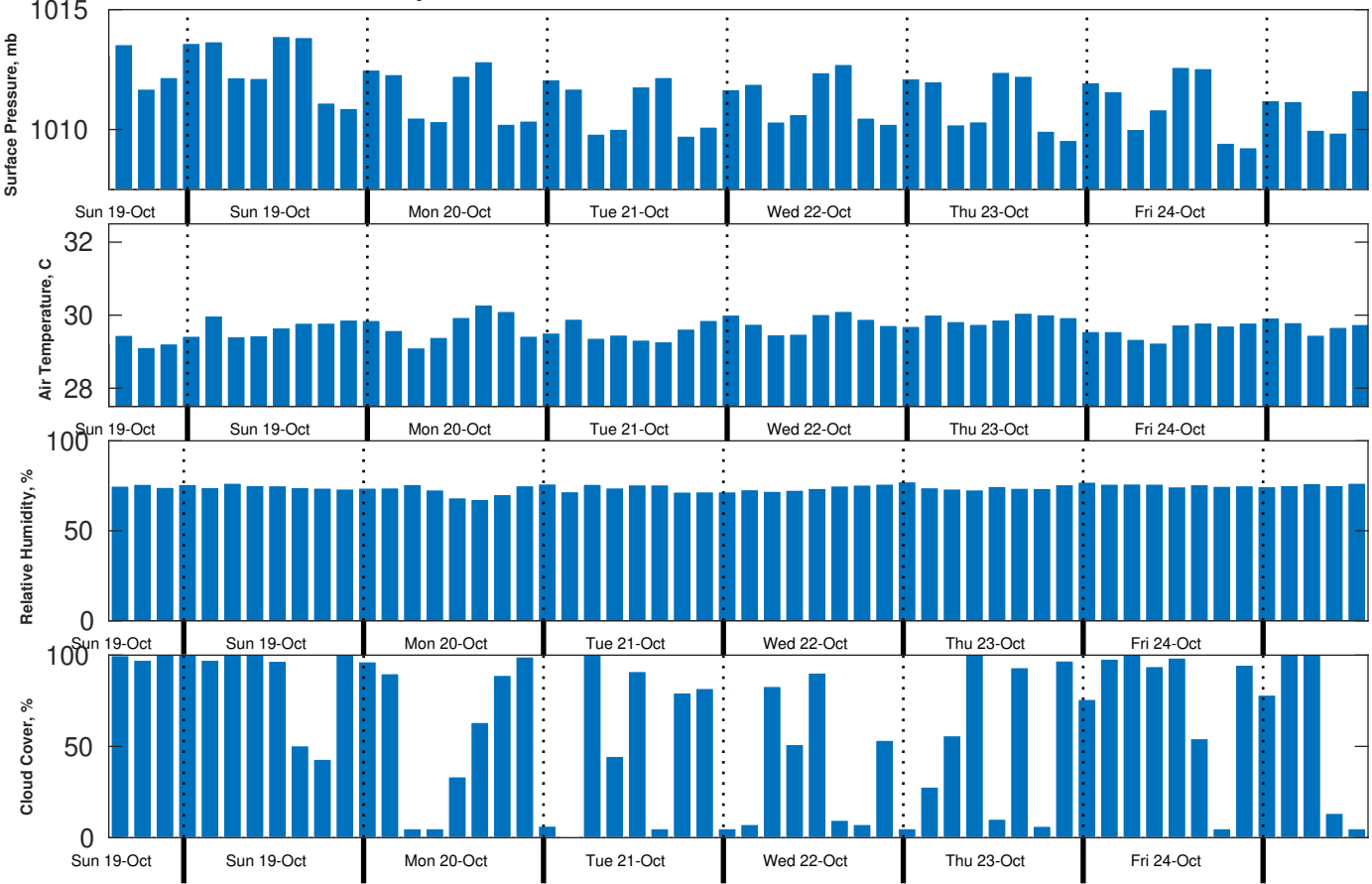
Met Forecast for Gyre from 19-Oct-2025 08:00:00 to 26-Oct-2025 08:00:00
