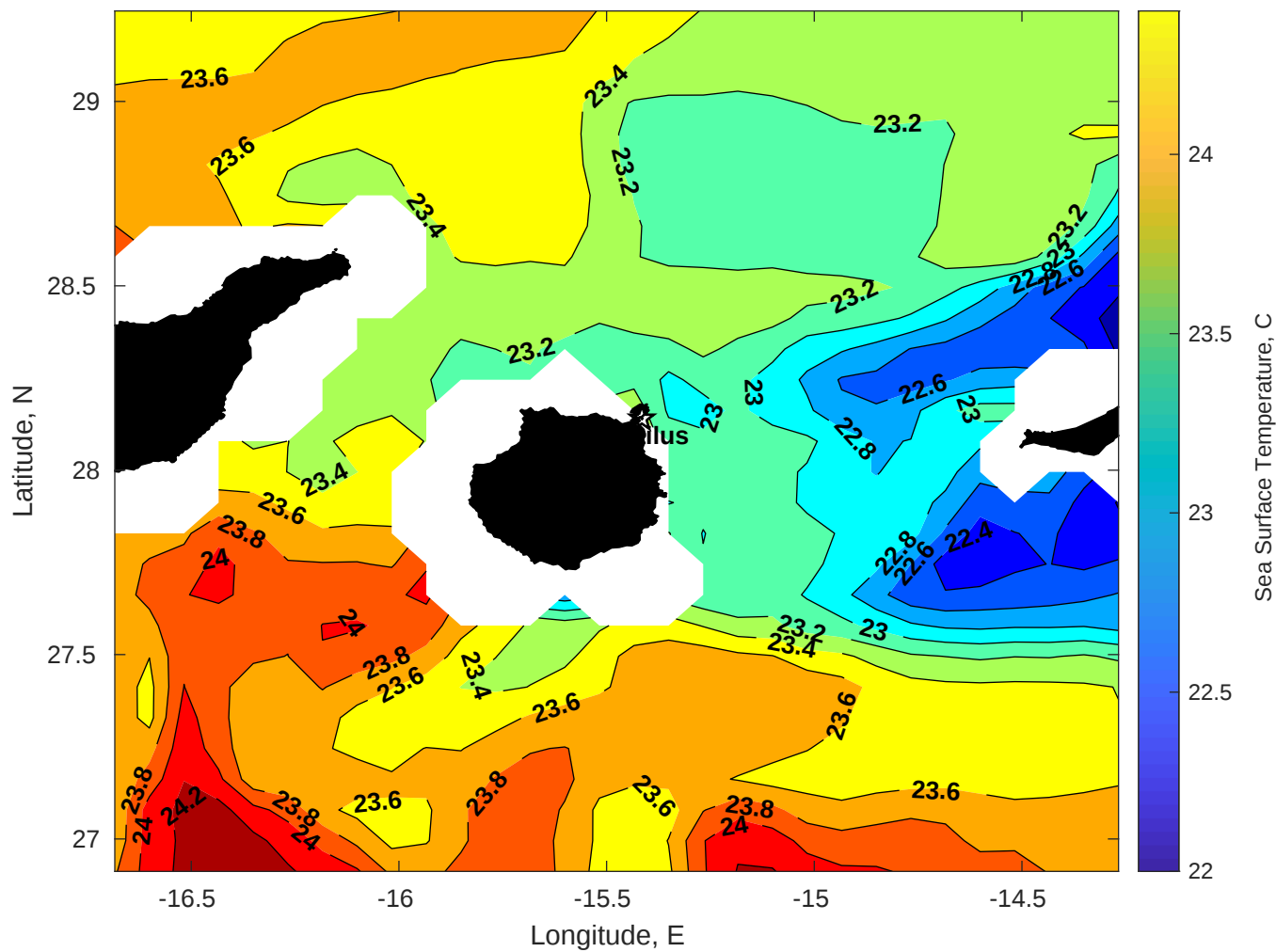
SST for Nautilus at 19-Oct-2025 00:00:00
